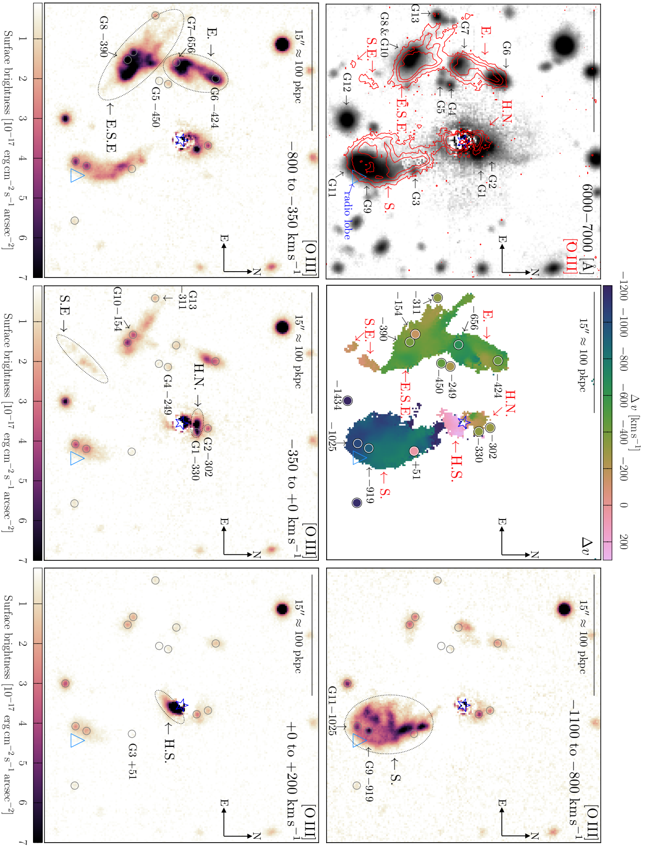
Figure 2. Top left: median flux over 6000–7000 Å in the MUSE datacube with [O III] surface brightness contours of 0.75, 2.5, and 5 \times 10^{-17} erg cm –2 s –1 arcsec –2 in red and with galaxies and nebulae labelled. Top middle: Map of the nebular line-of-sight velocities relative to the quasar. The positions of galaxies in the host group are marked by circles with line-of-sight velocity on the same scale. The top right panel and bottom row show narrow-band [O III] images extracted from the MUSE datacube over line-of-sight velocity intervals indicated in each panel. Nebulae are marked by ellipses and labelled while the quasar and radio lobe are marked by a blue star and triangle respectively. Galaxies are labelled if they fall within the displayed velocity interval.
