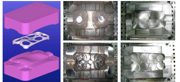
Fig. 4. Injection molding tooling produced by 3-axis Hybrid Layered Manufacturing (Gas Metal Arc Welding plus CNC machining): CAD model (left), near net shape molds (center), and finished molds (right) [317].
