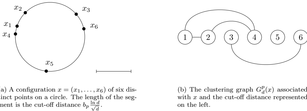
Figure 2: Example of a configuration of six points on a curve M isometric to a circle. The clustering partition of x = (x_1, \dots, x_6) is the partition of \{1, \dots, 6\} according to the connected components of the graph G_d^p(x) . Here it equals \mathcal{I}_d^p(x) = \{\{1, 2, 4\}, \{3, 6\}, \{5\}\} .
