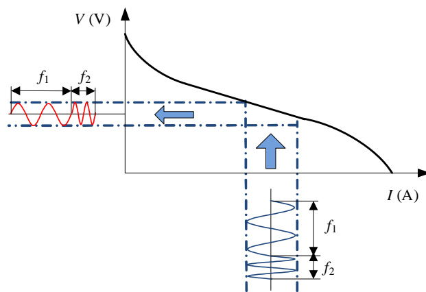
Fig. 4: Principle of the electrochemical impedance spectroscopy.
