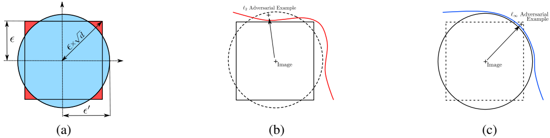
Figure 1: Left: 2D representation of the l_\infty and l_2 balls of respective radius \epsilon and \epsilon' . Middle: a classifier trained with l_\infty adversarial perturbations (materialized by the red line) remains vulnerable to l_2 attacks. Right: a classifier trained with l_2 adversarial perturbations (materialized by the blue line) remains vulnerable to l_\infty adversarial examples.
