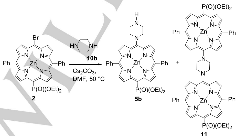
Scheme 5. S_NAr of bromoporphyrim 2 with piperazine ( 10b ) in DMF.
