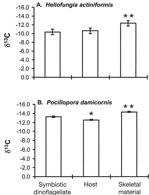
Fig. 2. \delta^{13}\text{C} of symbiotic dinoflagellate, host and skeletal organic material from (A) Heliofungia actiniformis and (B) Pocillopora damicornis . Each bar represents the mean \pm SE (all data within compartments pooled; n = 12 , H. actiniformis and n = 24 , P. damicornis ). Significant differences are indicated by asterisks (* p < 0.05 , ** p < 0.01 )
