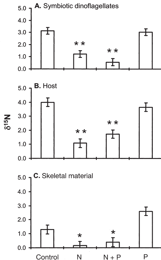
Fig. 4. \delta^{15}\text{N} of (A) symbiotic dinoflagellate, (B) host and (C) skeletal organic material of Pocillopora damicornis as a function of nutrient treatment. Each bar represents the mean \pm SE (n = 2 corals from 3 replicate patch reefs per treatment, i.e. n = 6). Significant differences are indicated by asterisks (*p < 0.05, **p < 0.01)
