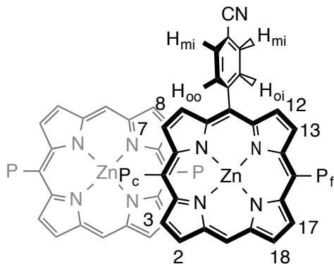
Chart 2. Numbering of protons in dimer (3d) 2 .
