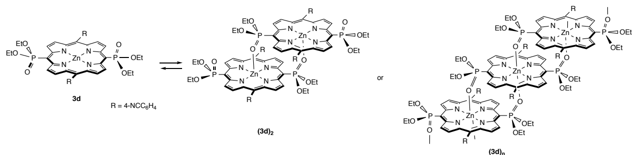
Scheme 2. Conversion between monomeric and aggregated redox active forms of porphyrin 3d in \text{CH}_2\text{Cl}_2 solution.
