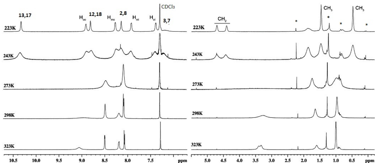
Figure 6. ^1\text{H} VT-NMR spectra of 3d in \text{CDCl}_3 at 223–323 K. Stars correspond to the signals of impurities.
