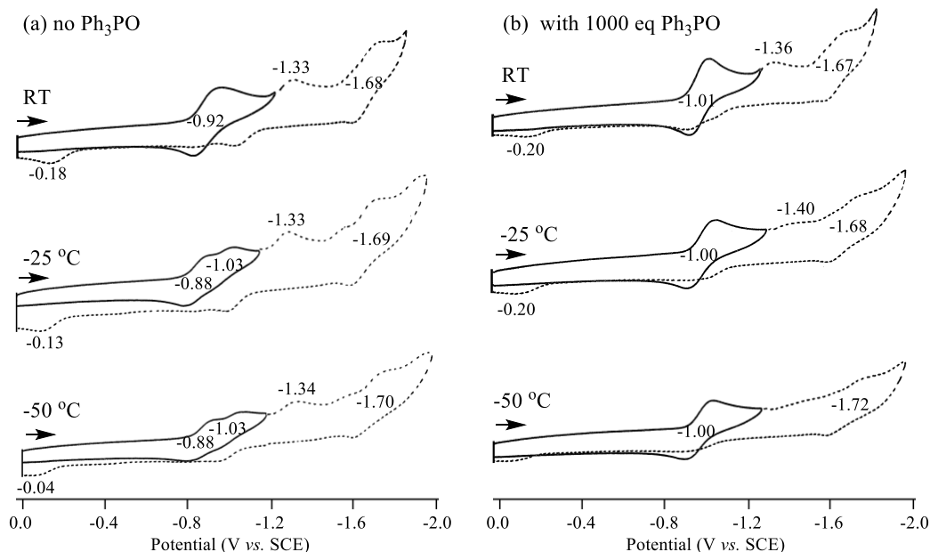
Figure 5. Cyclic voltammograms of 3d in \text{CH}_2\text{Cl}_2 at different temperatures before (a) and after (b) addition of 1000 eq of triphenylphosphine oxide ( \text{Ph}_3\text{PO} ).
