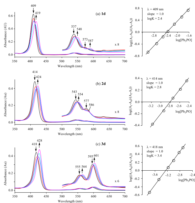
Figure 4. UV-vis spectral change of (a) 1d , (b) 2d and (c) 3d in CHCl 3 /MeOH (9:1) upon addition of Ph 3 PO. (Inset shows the Hill plots).
