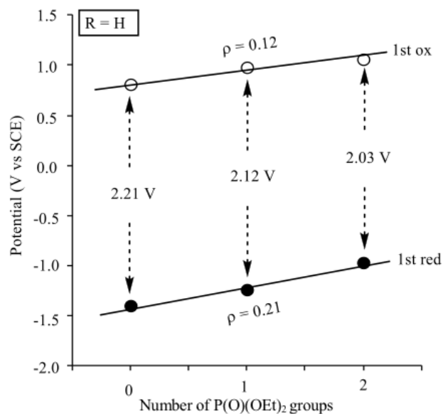
Figure 3. Correlation between number of \text{P}(\text{O})(\text{OEt})_2 groups on the porphyrin and the first reduction or oxidation of compounds 1c , 2c and 3c in PhCN, 0.1 M TBAP.
