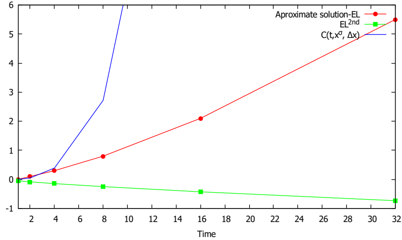
FIGURE 1. x_0 = 0, \Delta x_0 = 0.1, n = 5
