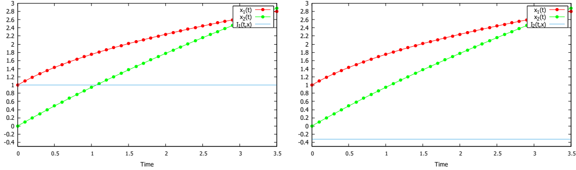
FIGURE 9. Simulation of the quantities I_1(t, x) and I_2(t, x) .
