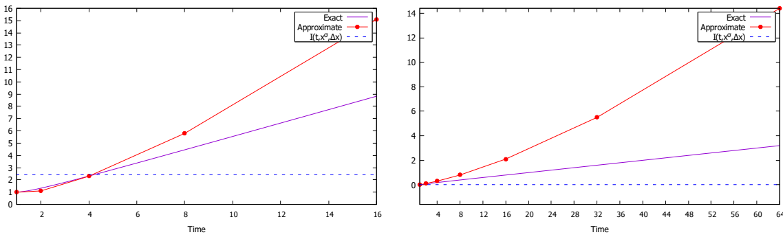
(A) x_0 = 1, \Delta x_0 = 0.1, n = 4
