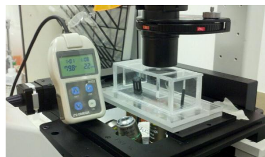
Figure 1: View of the Nikon Total Internal Reflection Fluorescence microscope with plexiglas humidity chamber and Omega RH32 humidity reader.
