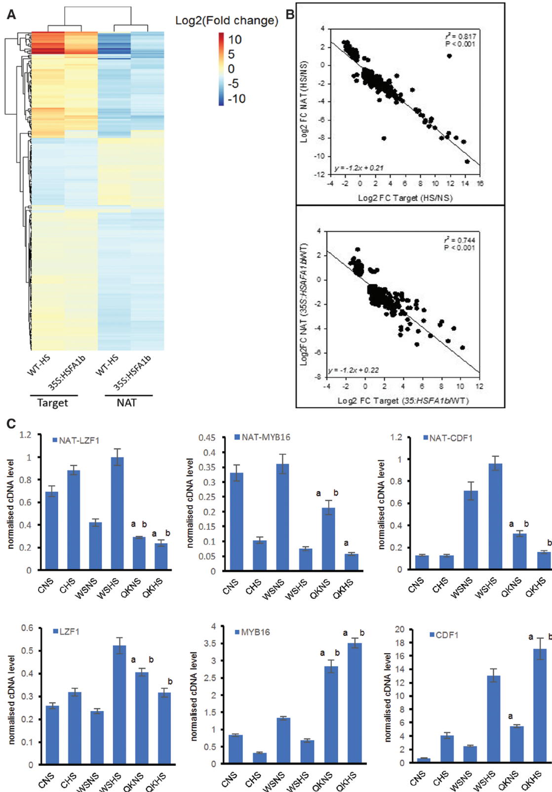
Fig. 6. HSFA1b regulates expression of cisNAT genes and their target sense genes. (A) Heat map showing differentially expressed cisNAT genes and their putative sense targets in WT plants in HS compared with NS and in 35S: HSFA1b NS plants compared with WT NS plants. (B) Linear correlation plots showing the relationship between cisNAT and sense target transcript abundance for WT plants subjected to HS compared with NS (top panel) and for 35S: HSFA1b NS plants compared with WT NS plants (bottom panel). (C) Transcript levels determined by qPCR of selected cisNAT genes and their TF gene sense target in HS and NS qKO plants compared with their parental genotypes as in the legend of Fig. 5B. The suffixes 'a' and 'b' are where the qKO mutant shows a significant difference ( P < 0.05 ) under the same conditions (NS or HS) from Col-0 (C) and Ws-0 (W) respectively.
