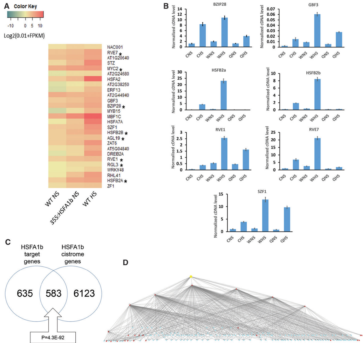
Fig. 5. HSFA1b can indirectly control expression through its regulation of TF gene expression. (A) Heat map comparing normalized FPKM values for 28 TF genes bound by HSFA1b and differentially expressed in 35S:HSFA1b and WT HS plants. Asterisks (*) indicate development-associated TF genes. (B) Confirmation of the regulation of selected TF genes by clade A1 HSF genes. Quantitative real-time RT-PCR was conducted on RNA from qKO rosettes under NS and HS in comparison with its parental genotypes Col-0 (C) and Ws-0 (W). The suffixes ‘a’ and ‘b’ are where the qKO mutant shows a significant difference ( P < 0.05 ) under the same conditions (NS or HS) from Col-0 and Ws-0, respectively. (C) Venn diagram showing the overlap between HSFA1b target genes scored from the ChIP-seq data (Supplementary Data S1) and the target genes bound by HSFA1b (HSF3) from the Arabidopsis Cistrome Atlas ( http://neomorph.salk.edu/dev/pages/shhuang/dap_web/pages/index.php ). The boxed callout number is the P -value for the significance of the overlap between the two data sets (hypergeometric distribution test). (D) An overview of a Cytoscape-generated HSFA1b hierarchical TF gene network using the data outputs from the Cistrome Atlas with the ChIP-seq and RNA-seq data from this study. The yellow node is HSFA1b, red nodes are TF genes bound by HSFA1b, and blue nodes are differentially expressed TF genes that respond to HS and HSFA1b overexpression, are not bound by HSFA1b, but are scored as binding to the red node TFs. An interactive version of this network is available as an interactive file (Supplementary Cytoscape File S1).
