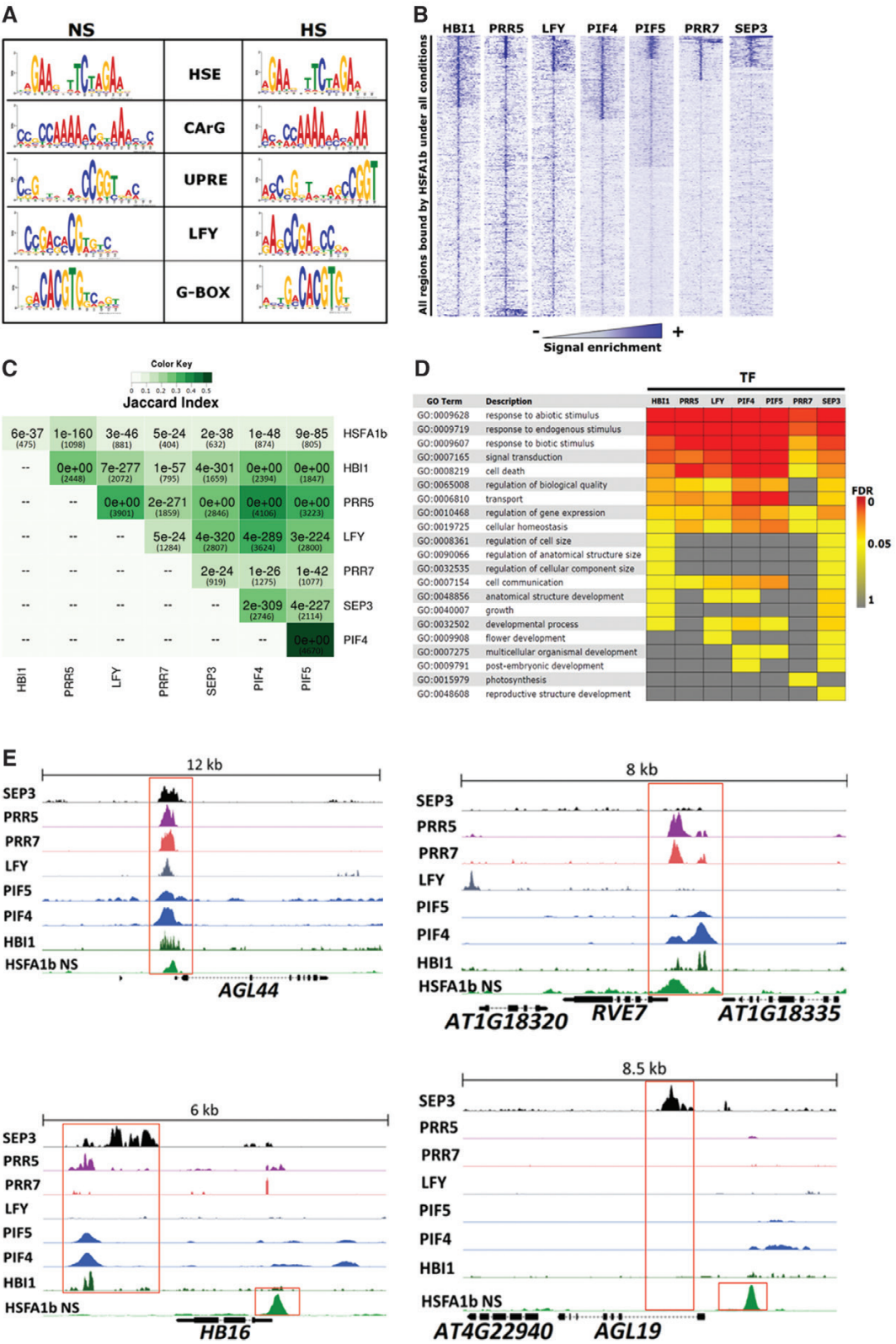
Fig. 7. Seven TFs co-ordinate with HSF1b. (A) All significant motifs within HSF1b peaks discovered by MEME ( P<0.0001 ) in the NS and HS data sets. (B) Density heat maps showing enrichment of ChIP-seq signals of the seven TFs on 10 kb around the regions bound by HSF1b. (C) Combined Jaccard index and pHYPER correlation matrix showing the significance of overlaps between the target genes of the seven TFs and HSF1b under NS conditions only. Numbers of genes in each overlap are in parentheses. (D) GO Slim analysis comparing the enriched Biological Process terms of the common targets between HSF1b and the other seven TFs. (E) Genome browser view of normalized ChIP-seq tags from the ChIP-seq data of the eight TFs showing examples of target genes bound by HSF1b and up to seven other TFs.
