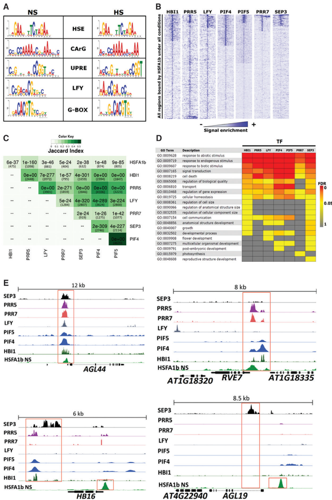
Fig. 7. Seven TFs co-ordinate with HSFA1b . (A) All significant motifs within HSFA1b peaks discovered by MEME ( P < 0.0001 ) in the NS and HS data sets. (B) Density heat maps showing enrichment of ChIP-seq signals of the seven TFs on 10 kb around the regions bound by HSFA1b . (C) Combined Jaccard index and pHYPER correlation matrix showing the significance of overlaps between the target genes of the seven TFs and HSFA1b under NS conditions only. Numbers of genes in each overlap are in parentheses. (D) GO Slim analysis comparing the enriched Biological Process terms of the common targets between HSFA1b and the other seven TFs. (E) Genome browser view of normalized ChIP-seq tags from the ChIP-seq data of the eight TFs showing examples of target genes bound by HSFA1b and up to seven other TFs.
