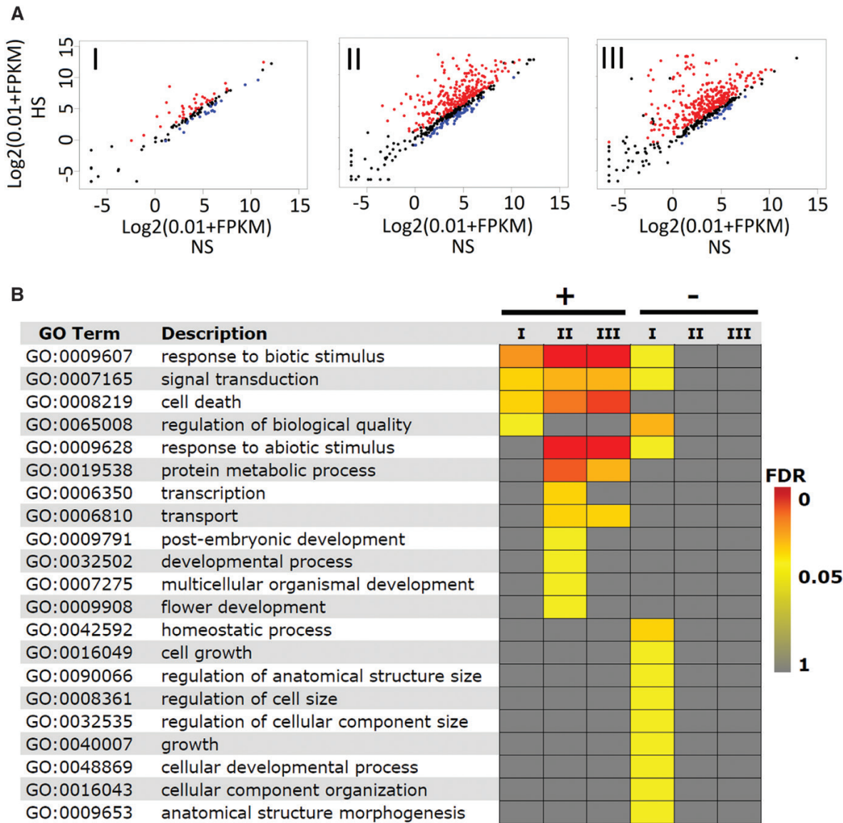
Fig. 3. Most HSFA1b target genes are responsive to HS. (A) Scatter plots of transcript abundance of HSFA1b target genes in response to HS. Red and blue dots represent up- and down-regulated genes, respectively ( q \leq 0.05 ), and black dots show genes with expression q > 0.05 . The numbers shown in each panel are the number of DEGs in each group. (B) GO Slim analysis heat map comparing the enriched BP terms of up- (+) and down- (-) regulated HS-responsive genes in Groups I–III (Benjamini–Hochberg FDR < 0.05 ).
