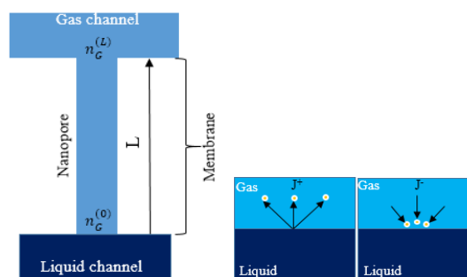
Fig. 2. Convection – diffusion transfer mechanism inside the overlapping meandering channels.
