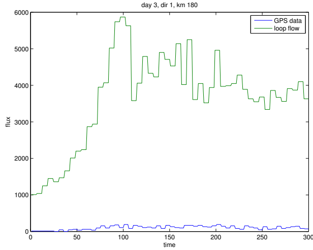
Figure 6: Loop detectors data (6 minutes average, green) and GPS data (blue). March 19, direction 1, km 180.
