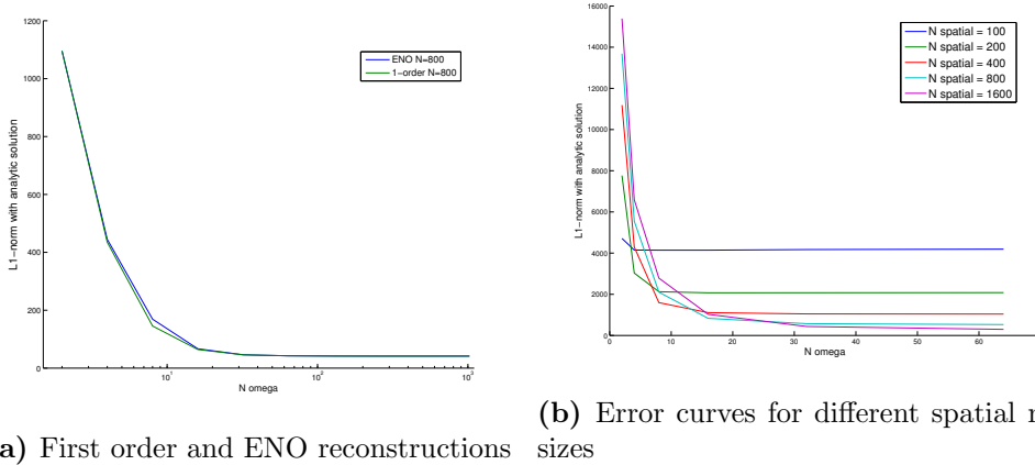
Figure 11: Convergence analysis in the probabilistic direction.
