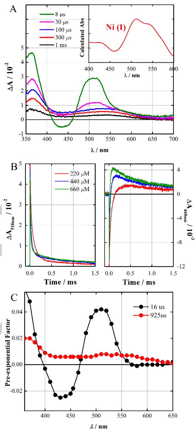
Figure 7. (A) Transient absorption spectra of 24 μM [Ru(bpy) 3 ] 2+ , 660 μM catalyst 1, in Ar-purged 1:1 solvent mixture of ACN and aqueous ascorbate/ascorbic acid buffer (pH 4; 0.1 M) at the indicated delay times after excitation. Laser energy = 8 mJ, λ exc at 460 nm. Inset: DFT-optimised UV-Vis spectrum of Ni I (catalyst 1), see SI for more details. (B) Corresponding transient absorption kinetics at 510 nm (left) due to the decay of Ru I and 440 nm (right) due to the growth of Ni I (catalyst 1) as a function of catalyst concentration (C) Decay associated spectra (DAS) of the transient absorption kinetics of catalyst 1 (same conditions as part A). Black lines correspond to [(Ru I + Asc + ) - (Ru II + Asc)] while the red lines correspond to [(Ni I + Asc + ) - (Ni II + Asc)], with their respective lifetimes.
