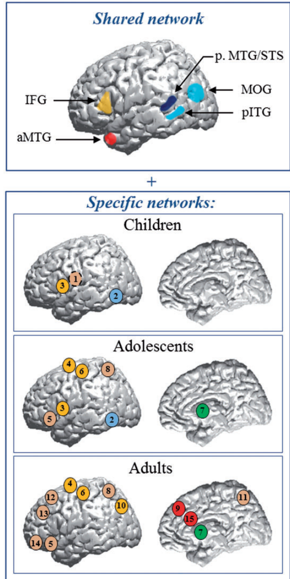
Fig. 5. Neural correlates of social interaction recognition across development. This figure summarizes the group analysis results of the fMRI study, in the children, adolescent and adult groups. The table (left) describes the regions activated during the observation of SI vs NM in our study, and the findings from other studies: activation during human motion (HM) or SI observations. At the group level, regions which showed increased activation for SI > NM are indicated in color, and with a "+" for when remaining significant at the cluster level. The "x" sign indicates the regions revealed in the group comparison for the contrast SI > NM. The illustrations (right) present the networks shared by the three groups (top panel) and regions specific to each group. Numbers correspond to the regions indicated in the table. The brain regions involved in visual perception are represented in light blue, in the mirror system in yellow, in the social brain in red, and regions involved in these three networks are in dark blue. The caudate nucleus is indicated in green, and other regions are represented with brown color. g.: gyrus, sup.: superior, Ado.: adolescents.
