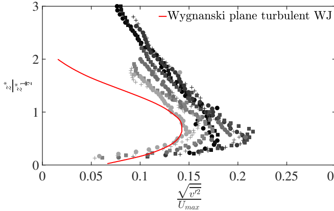
(b) Turbulence intensity in the normal direction
