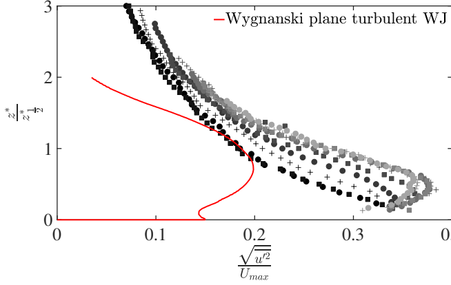
(a) Turbulence intensity in the streamwise direction
