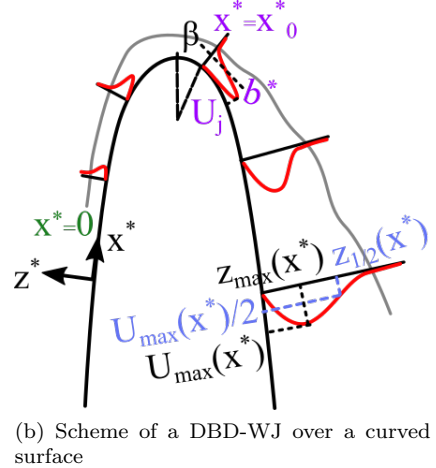
Figure 7: (a) \theta^* angle definition over a cylinder, (b) Scheme of a DBD-WJ over a rounded trailing-edge and its specific variables
