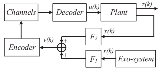
Fig. 1: System setup
