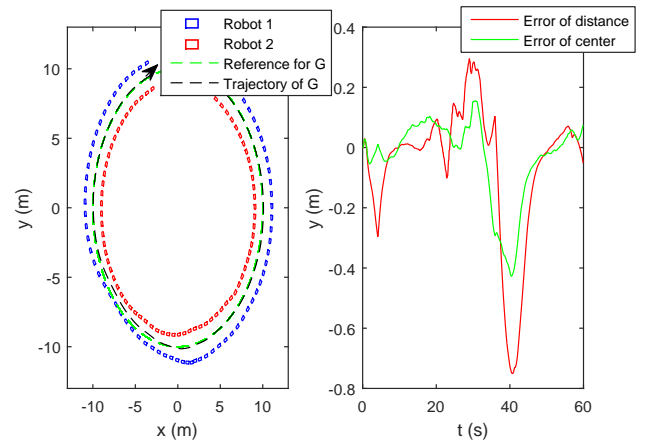
Fig. 8: Tracking performance of extended results in [30]
