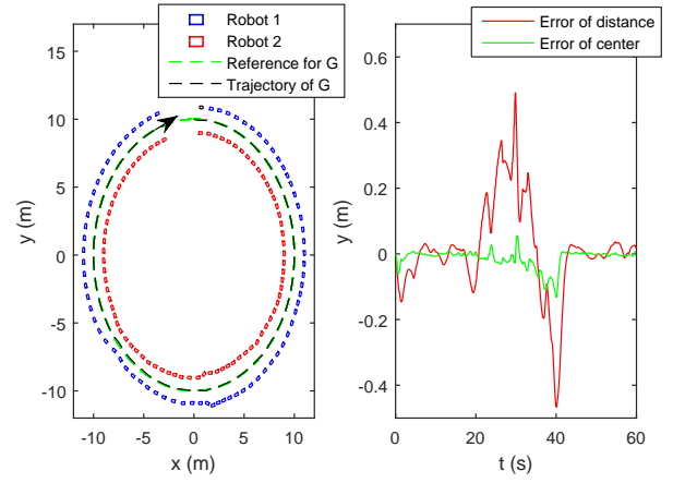
Fig. 6: Tracking performance with LQ performance to Case 1
