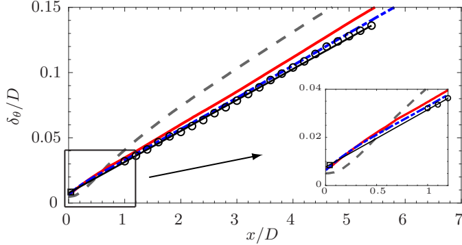
FIGURE 12. (Colour online) Profiles of the shear-layer momentum thickness \delta_\theta : experiment ( \square hot-wire, \circ PIV, — linear interpolation), extended baseline LES 10M ( - - - ) and extended LES with nozzle-interior turbulence modelling BL16M_WM_Turb ( — ) and BL69M_WM_Turb ( - . - ).
