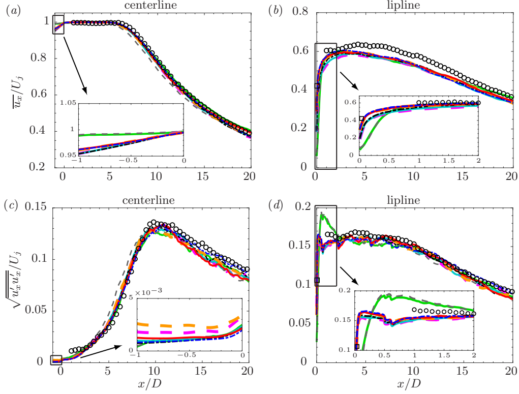
FIGURE 7. (Colour online) Profiles along the centerline and lipline of (a,b) mean and (c,d) RMS streamwise velocity: experiment ( \square hot-wire, \circ PIV), baseline LES 10M (---) and 64M (—), and LES with nozzle-interior turbulence modelling BL16M (—·—), BL16M_Turb2 (—·—), BL16M_Turb (—), BL16M_WM (—·—), BL16M_WM_Turb2 (—·—) and BL16M_WM_Turb (—).
