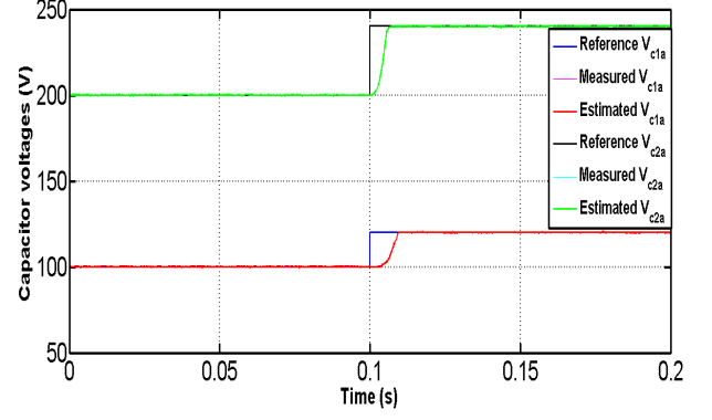
Figure 7: Floating capacitor voltages: V_{c1a-ref} , V_{c1a} , \hat{V}_{c1a} and V_{c2a-ref} , V_{c2a} , \hat{V}_{c2a} with DC bus variation.
