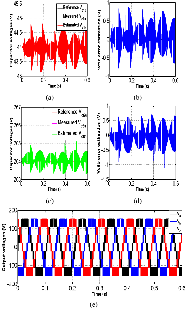
Figure 11: Simulation results in case of a 7-cells 8-levels FCI.
