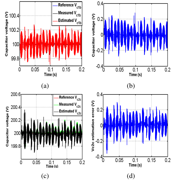
Figure 8: Floating capacitor voltages.
