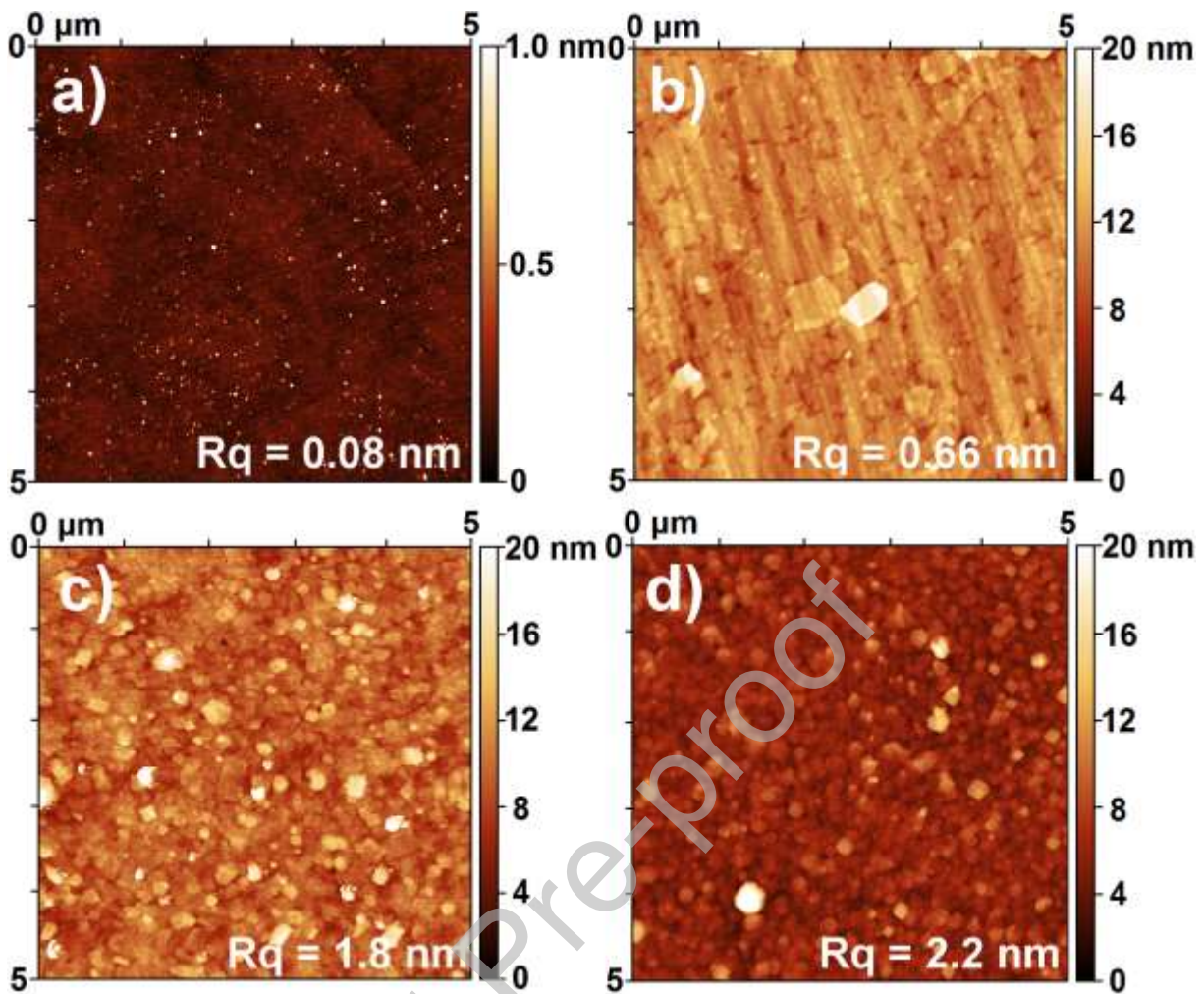
Fig. 3. AFM images of a) the STO substrate, b) the monolayer film of \text{Ca}_2\text{Nb}_3\text{O}_{10}^- -NS deposited on glass by Langmuir-Blodgett method, c) the KNO/STO film, d) the KN/ \text{Ca}_2\text{Nb}_3\text{O}_{10}^- -NS/glass film.
