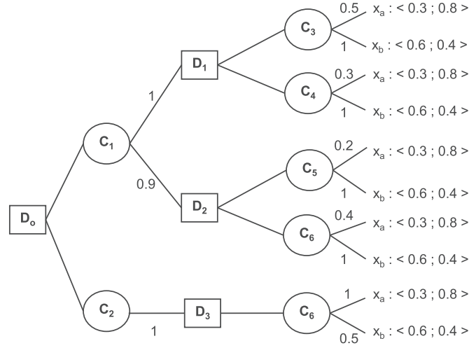
Fig. 2. Collective possibilistic decision tree of Example 3.
