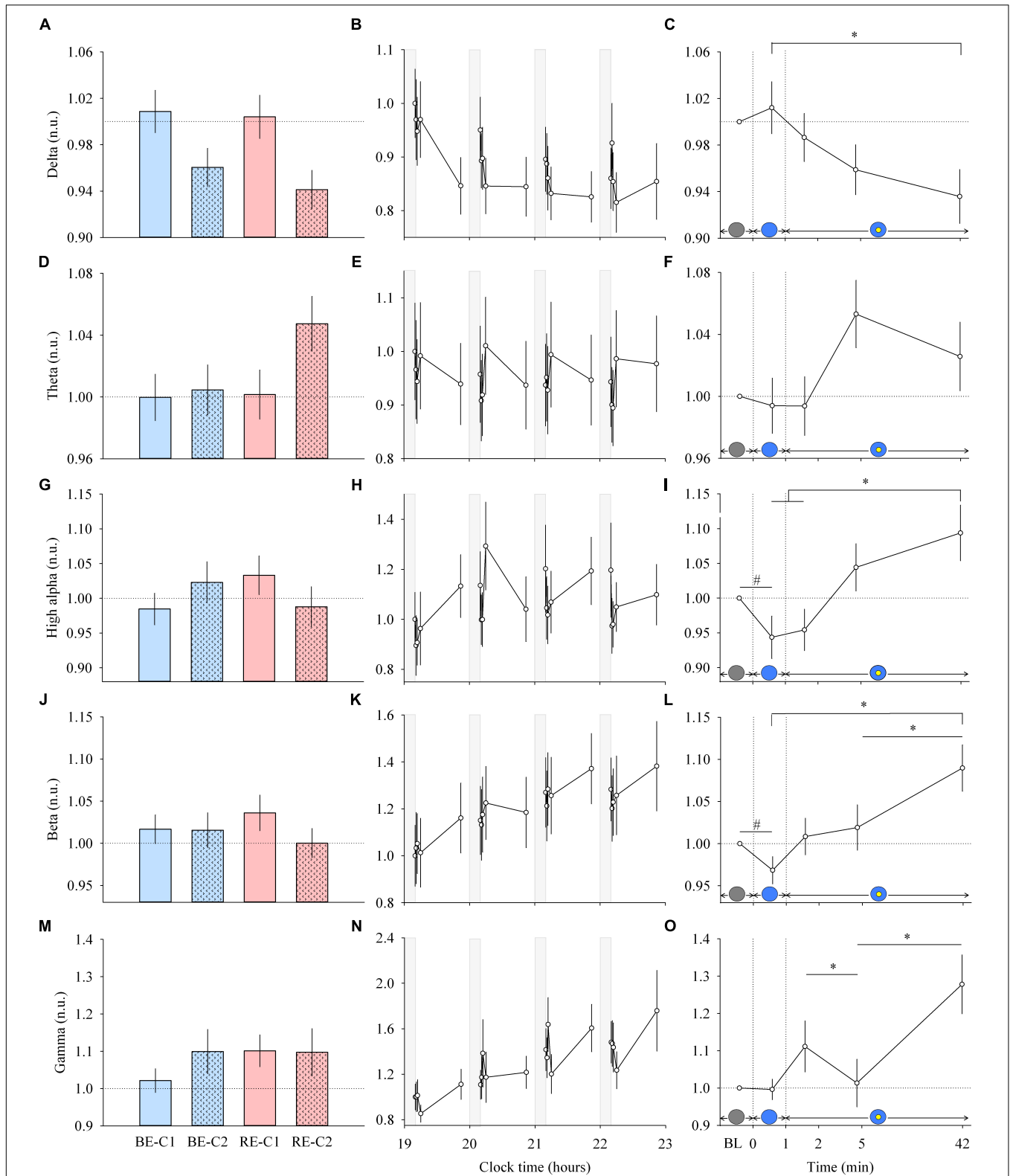
FIGURE 2 | EEG response and dynamics during light exposure. (A,D,G,J,M; left column) Effect of light condition on each EEG band. EEG delta, theta, high alpha, beta and gamma absolute power densities are expressed relative to their respective dim light (min 0) values, in normalized units (n.u.). (B,E,H,K,N; middle column) Variation of EEG delta, theta, high alpha, beta, gamma during the protocol. Each pulse, corresponding to the average over the four light conditions, is shown in plain lines. Absolute EEG power densities for each band are expressed relative to their dim light level at 19:10, in normalized units (n.u.). Gray bars show the 10-min (Continued)
