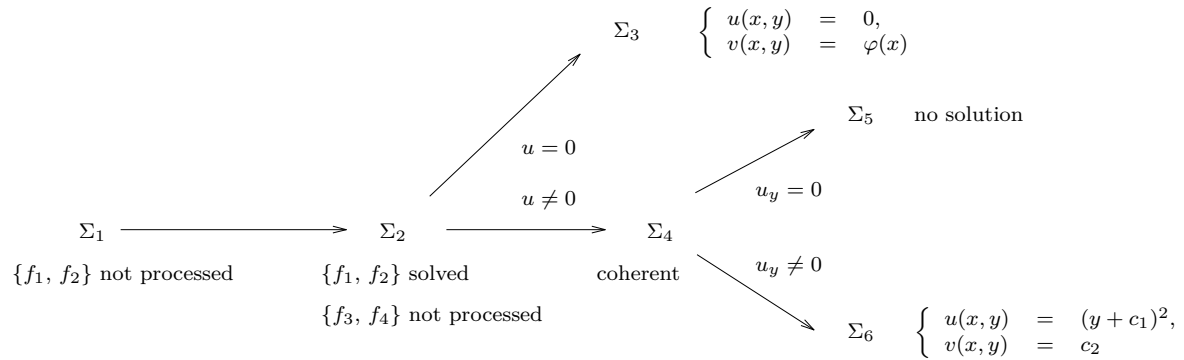
Figure 3: The splitting tree of Section 3.4.2.
