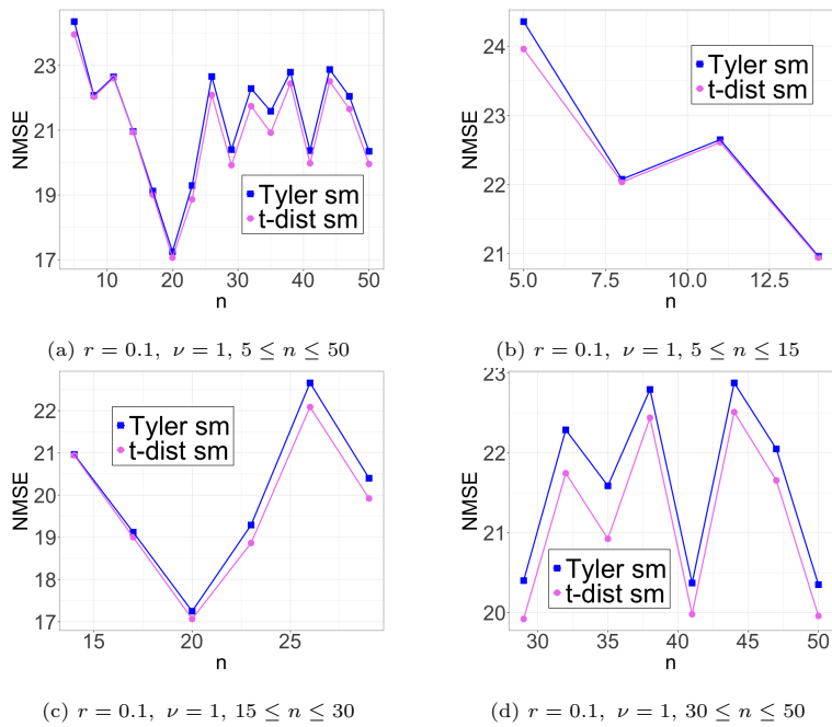
Figure 2: Multivariate t -distribution with AR( r ) covariance structure ( p = 50, r = 0.1, \nu = 1 and \boldsymbol{\mu} is set to a vector of 5): comparison of NMSE(\boldsymbol{\Sigma}) for "Tyler sm" and "t-dist sm" algorithms when the mean is fixed to the sample mean. Normalized mean squared-errors are computed over 100 simulated samples of n observations each. Varying values of n from 5 to 50 (a) are also plotted separately for better layout in (b,c,d).
