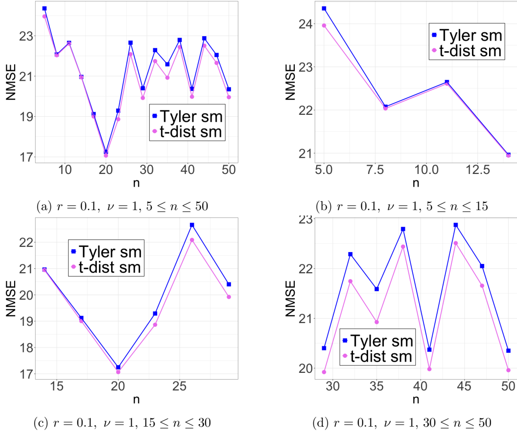
Figure 2: Multivariate t -distribution with AR( r ) covariance structure ( p = 50, r = 0.1, \nu = 1 and \boldsymbol{\mu} is set to a vector of 5): comparison of NMSE(\boldsymbol{\Sigma}) for "Tyler sm" and "t-dist sm" algorithms when the mean is fixed to the sample mean. Normalized mean squared-errors are computed over 100 simulated samples of n observations each. Varying values of n from 5 to 50 (a) are also plotted separately for better layout in (b,c,d).
