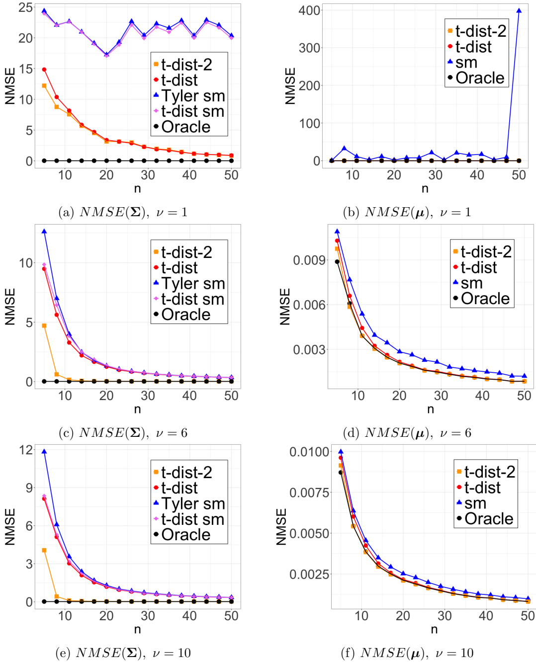
Figure 1: Multivariate t -distribution with AR( r ) covariance structure ( p = 50, r = 0.1, \nu \in \{1, 6, 10\} and \mu is set to a vector of 5). Normalized mean squared-errors for \Sigma (first column) and \mu (second column) are computed over 100 simulated samples of n observations each with n varying from 5 to 50.
