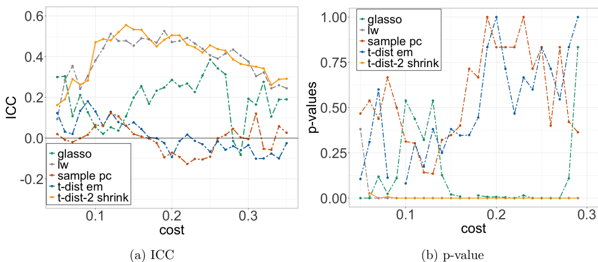
Figure 5: Intraclass correlation coefficient (ICC) between two fMRI sessions ( S_{11} and S_{22} ) (a) and associated p-values (b) with respect to the pre-set percentage of edges in the graphs (cost). The ICC values are shown for the various estimators considered in this study. The larger the ICC, the higher the consistency between the two sessions and the higher the estimator reliability.
