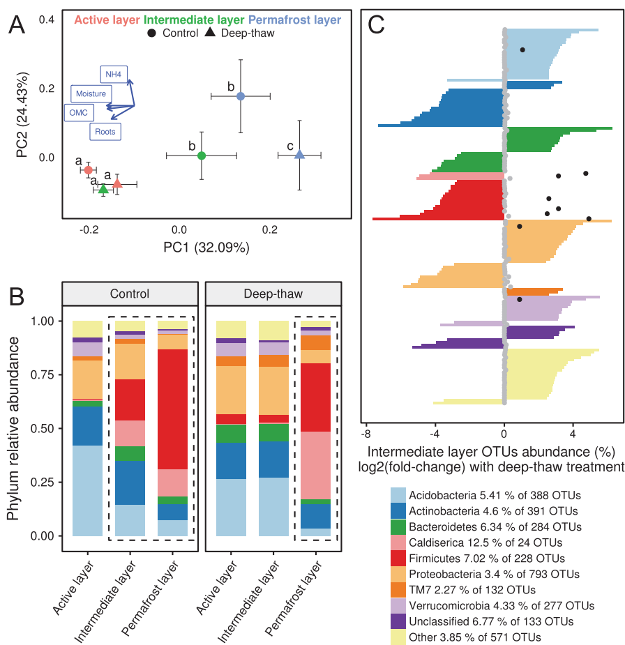
Fig. 1 Bacterial community structure based on 16S rRNA V3 region. a Principal coordinates analysis of weighted UniFrac distances; markers and error bars represent mean and standard error, respectively, of coordinates on the ordination axes for each depth \times treatment combination ( n = 6 , except intermediate layer–deep thaw where n = 5 ); different letters denote significantly different communities ( manyglm post hoc, see SI Table S4). b Mean relative abundance of phyla in each depth \times treatment combination; dashed rectangles enclose permanently frozen samples. c
