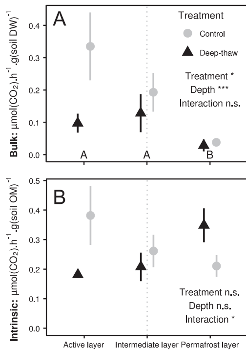
Fig. 2 Potential aerobic respiration of soils from different depths in control and decadal in situ deep-thaw plots during laboratory incubation at 11 °C, measured for 1 week after 1 month pre-incubation, expressed per gram soil dry weight (a) and per gram soil organic matter (b); samples to the right of the dotted line are from permanently frozen soil layers; means ± SE ( n = 6). Asterisks denote significant effects (* P < 0.05; *** P < 0.001; n.s. non significant), letters denote significant differences between depths
