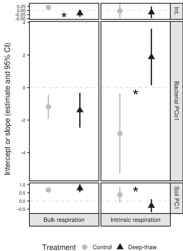
Fig. 3 Intercepts and slopes (95% CI) of the best-fitting multiple linear regressions of respiration against soil chemistry (soil PC1) and bacterial community structure (bacterial PCo1). Asterisks denote significant differences between treatments ( P < 0.05). Int. intercept
