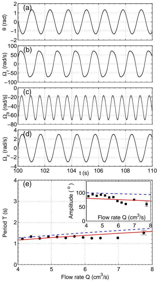
FIG. 4. Typical solutions of equations (5) and (6) numerically integrated with \tau_a = 0.63 s, \tau_b = 1.70 s, r/R = 0.25 , U_a/r = 123 s ^{-1} and \Omega_{r0}^2 = (g/R) \sin \alpha = 36.9 s ^{-2} ; (a) oscillatory motion \theta(t) obtained at long time scales, (b)-(d) related oscillations of the angular velocities \Omega_r(t) , \Omega_\theta(t) and \Omega_z(t) . (e) Time period of the drop oscillations versus flow rate. Inset: amplitude versus flow rate. Lines show theoretical predictions integrating Eqs. (5) and (6). Straight line \alpha = 1.1^\circ , dashed line \alpha = 1.0^\circ .
