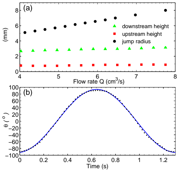
FIG. 2. Measured for a plate inclination of \alpha \approx 1.0 \pm 0.1^\circ : (a) Radius of the hydraulic jump (circle), upstream (square) and downstream (triangle) fluid heights around the jump, versus flow rate. (b) Typical law \theta(t) for the drop motion, \theta being the drop angular position defined with respect to the lowest point of the jump (unstable equilibrium position). The line is a fit with a cosine function.
