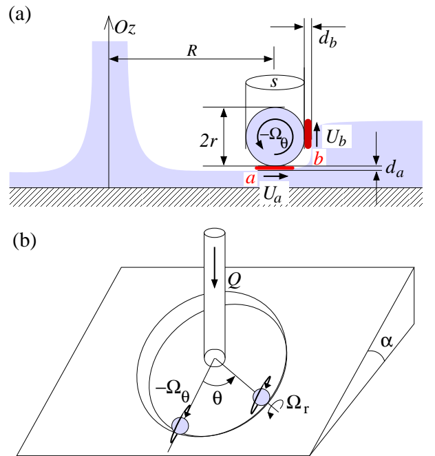
FIG. 3. (a) Sketch of the drop and fluid motion expected in a radial vertical plane containing the jump central axis. The drop is rotating very fast because of the shear stress transmitted across the air film. (b) Principle of the instability viewed in three dimensions. The drop, when pushed from the lowest point of the jump, tries to keep constant its angular momentum, which develops an active radial component of the rotation rate vector that tends to amplify the drop displacement.
