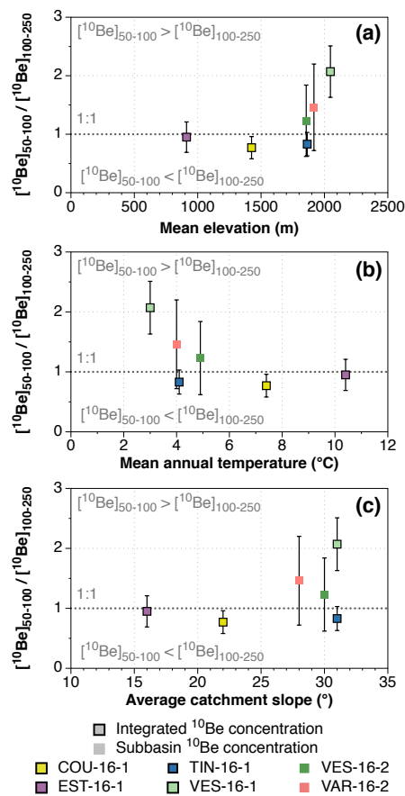
5 Figure 5: Differences in ^{10}\text{Be} concentrations of the 50–100 and 100–250 \mu\text{m} size fractions as a function of (a) elevation, (b) mean annual temperature and (c) average subbasin slope. Mean elevation and temperature were calculated for quartz-bearing surfaces only using a 5 m resolution DEM from the Institut National de l'Information Géographique et Forestière ( http://professionnels.ign.fr/donnees ). Temperature data are from the WorldClim database ( http://worldclim.org/version2 ; Fick and Hijmans, 2017). Subbasin concentrations (Table 2) are used for VES-16-2 and VAR-16-2 to exclude their nested upstream subbasins (VES-16-1 and COU-16-1, respectively).
