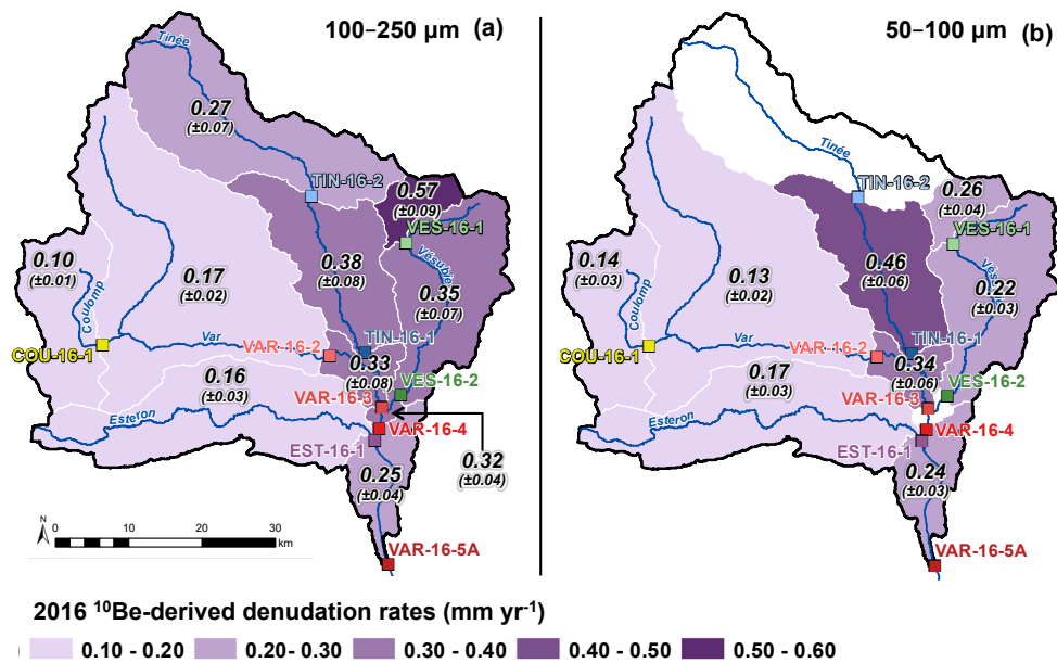
Figure 3: Spatial variations of 10 Be-derived denudation rates for the 2016 Var samples (data reported in Table 1). White polygons denote the absence of data. Denudation rates were derived from the (a) 100–250 μm and (b) 50–100 μm grain size fractions.
