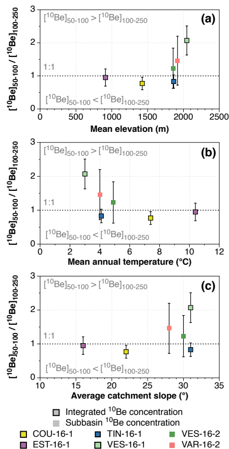
5 Figure 5: Differences in ^{10}\text{Be} concentrations of the 50–100 and 100–250 \mu\text{m} size fractions as a function of (a) elevation, (b) mean annual temperature and (c) average subbasin slope. Mean elevation and temperature were calculated for quartz-bearing surfaces only using a 5 m resolution DEM from the Institut National de l'Information Géographique et Forestière ( http://professionnels.ign.fr/donnees ). Temperature data are from the WorldClim database ( http://worldclim.org/version2 ; Fick and Hijmans, 2017). Subbasin concentrations (Table 2) are used for VES-16-2 and VAR-16-2 to exclude their nested upstream subbasins (VES-16-1 and COU-16-1, respectively).
