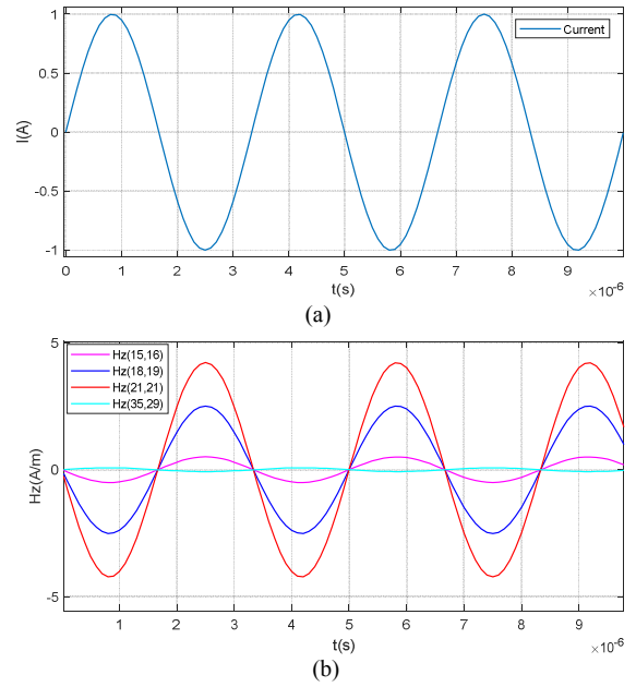
Fig. 4. (a) Excitation current, (b) Calculated H_z component at different positions.
