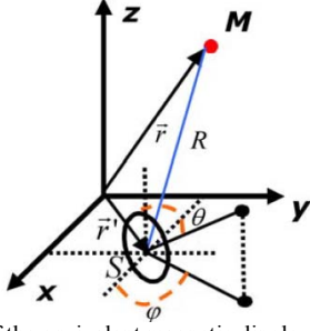
Fig. 2. Definition of the equivalent magnetic dipole.
