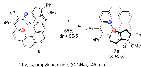
Scheme 8. Synthesis of the helical thiophosphinate 7a and acid 8a via regio- and diastereoselective photocyclization of the thiophosphinate 6 .
