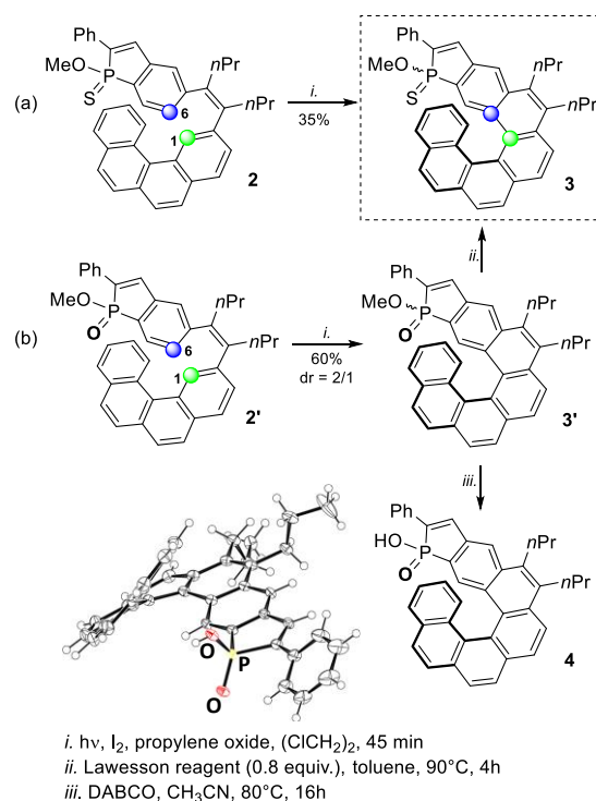
Scheme 4. Two alternative pathways (a, b) for the synthesis of the helical methyl thiophosphinate 3 . And X-ray crystal structure of the phosphinic acid 4 . Note: In compound 4 , the phosphorus center is not stereogenic, due to H-shift between the two oxygens.
