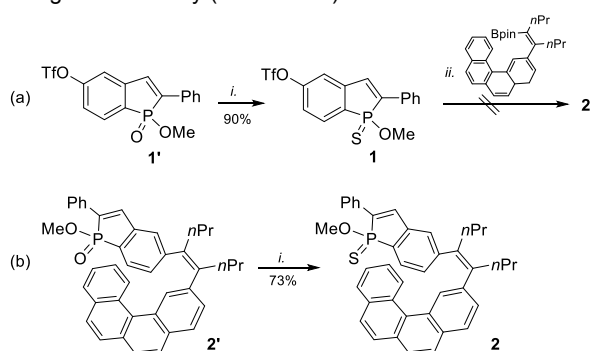
Scheme 3 Synthesis of olefin 2 displaying a thiophosphinate function.
