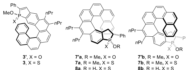
Figure 2. Overview of the phosphinic/thiophosphinic acids and esters obtained in this work.
