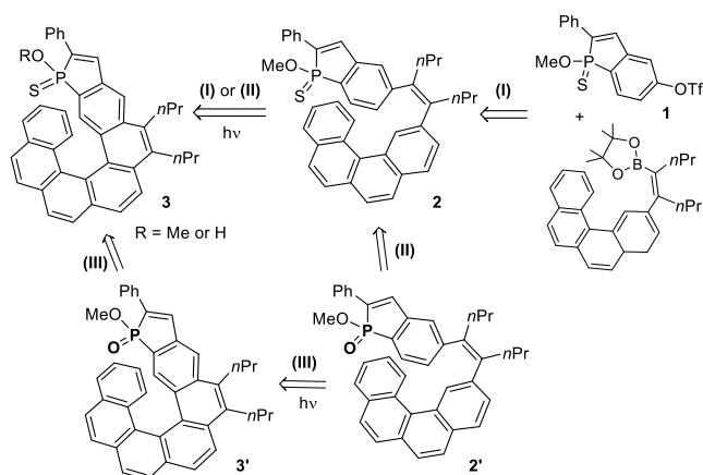
Scheme 2. Retrosynthetic approaches to 3 via the oxidative photocyclization method: paths (I), (II) and (III).
