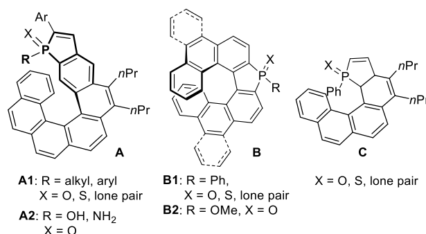
Scheme 1 Representative phosphahelicenes from the literature.
