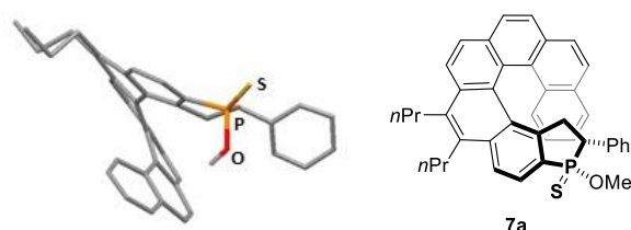
Figure 1. Crystal structure of the helical thiophosphinate 7a .
