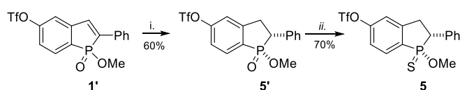
Scheme 5 Synthesis of 5 via chemo- and diastereoselective hydrogenation of 1' and subsequent O/S exchange.
