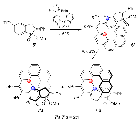
Scheme 5 Synthesis of 5 via chemo- and diastereoselective hydrogenation of 1' and subsequent O/S exchange.
