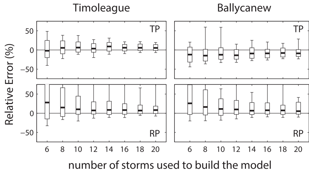
Figure 7. Sensitivity of the annual load estimations to the number of events initially used to calibrate nonlinear model M3 at Timoleague and Ballycanew (500 random draws).
