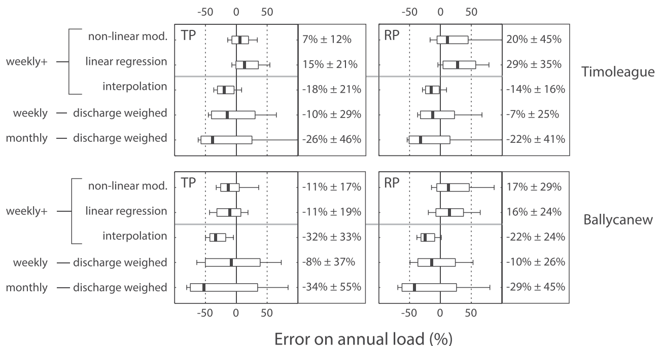
Figure 6. TP and RP relative errors on annual load estimations using nonlinear modeling, a simple linear regression model, interpolation based on a weekly+ survey, and discharge weighted method based on weekly or monthly sampling strategies. Relative bias ± s.d. errors are indicated on the right axis of each plot.
