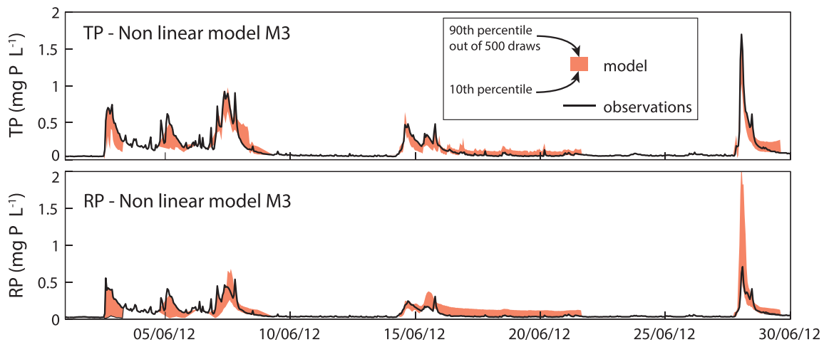
Figure 5. Example of continuous TP and RP concentration series after storm reconstruction based on the nonlinear model M3, during June 2012 in the Timoleague catchment.
