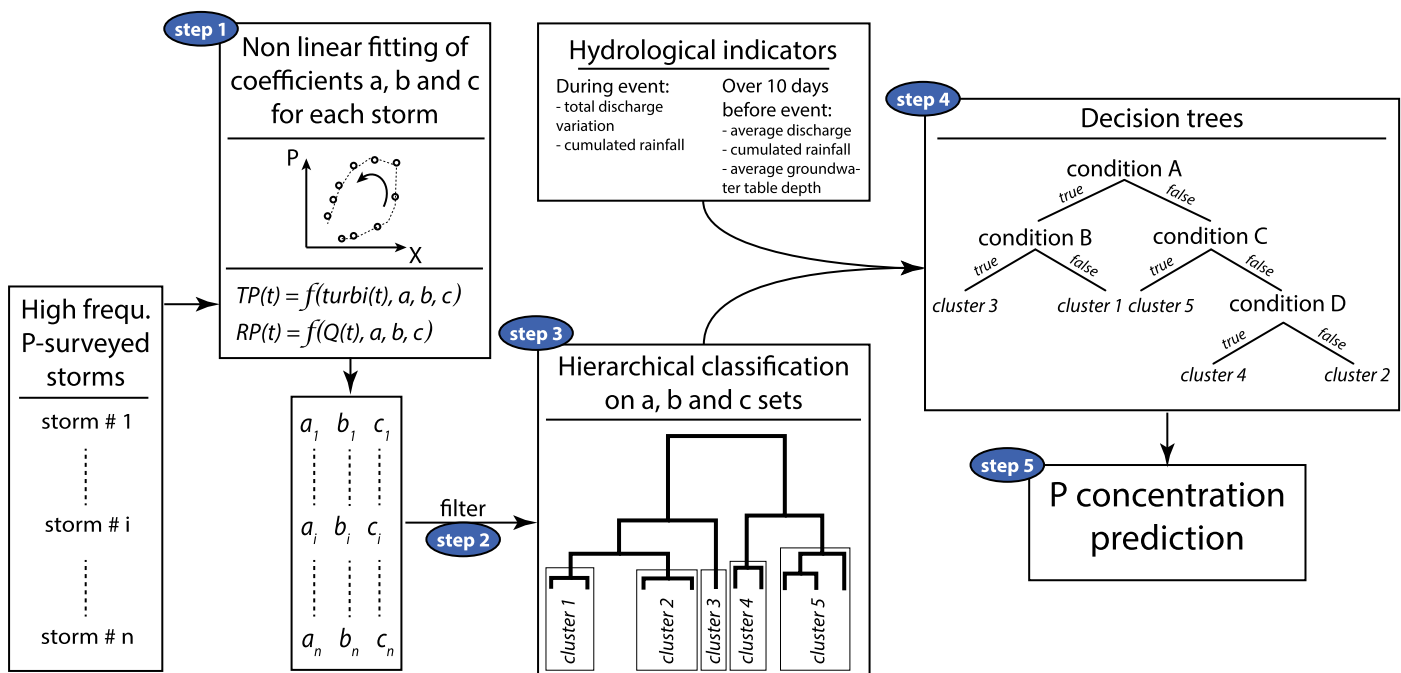
Figure 3. Successive steps for building nonlinear empirical models.
