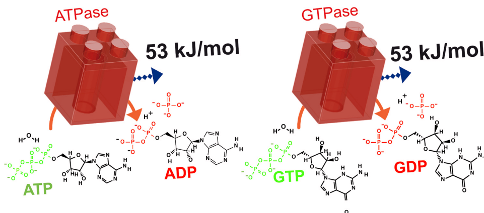
Figure 1. ATP and GTP hydrolysis release the same quantity of energy. ATPases and GTPases hydrolyse their NTP substrates to NDP and inorganic phosphate; both hydrolysis reactions liberate 53 kJ/mol Gibbs free energy. ATP, adenosine 5'-triphosphate; GTP, guanosine 5'-triphosphate; NTP, nucleoside triphosphate; NDP, nucleoside diphosphate; \text{P}_i , inorganic phosphate.
