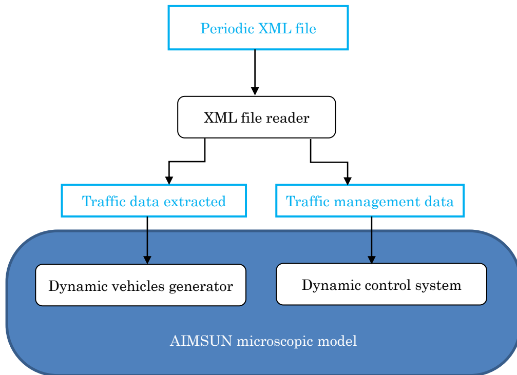
Figure 4 – Development architecture
