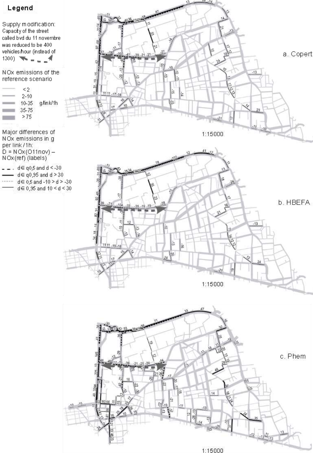
Figure 3: impact of the O11nov scenario on the estimated NOx emissions. NOx emissions of the reference scenario is figured in ligh grey, major differences of O11nov to the reference in dark. More explanations of method in the text.
