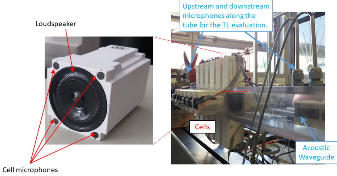
FIG. 7. Left: Unit cell. Right: Prespective of the lined waveguide, with upstream and downstream microphones for the TL evaluation through the transfer matrix method.
