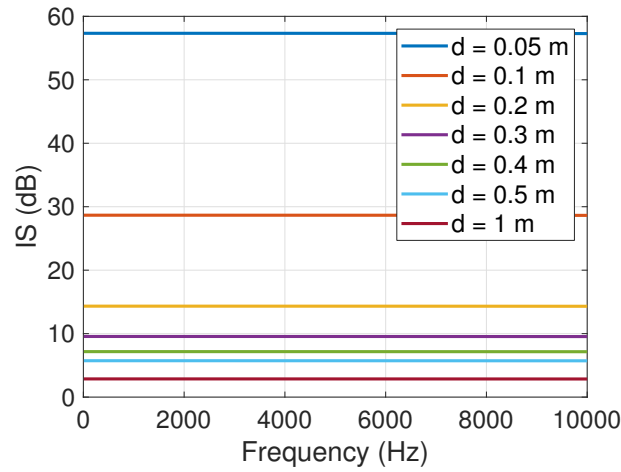
FIG. 4. Isolation (in dB) as a function of frequency, for different values of the parameter d .
