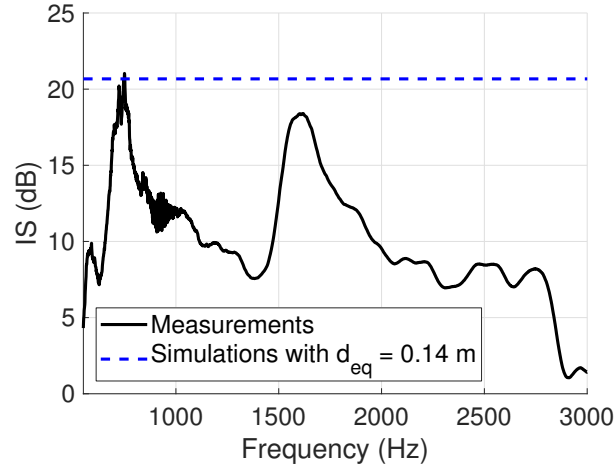
FIG. 9. Isolation index: measurements compared to 1D reduced model simulation with d equivalent to the experimental application.
