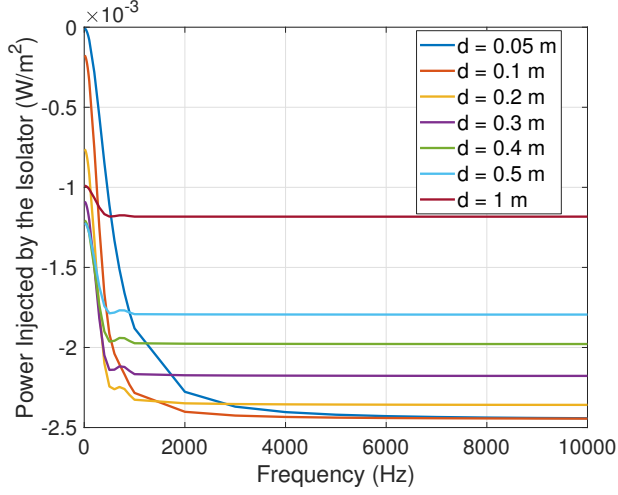
FIG. 5. Acoustic power injected by the isolator into the acoustic domain, as a function of frequency, for different values of the parameter d , in case of an incident wave of 1Pa RMS in the positive x direction.
