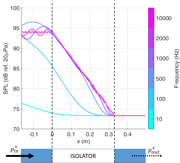
FIG. 6. Sound pressure level (in dB ref. 20\mu Pa) along the system for different frequencies, in case of an incident wave of 1 Pa RMS in the positive x direction. Parameter d = 0.14 m. The isolator is located between x = 0 and x = 0.33 m
