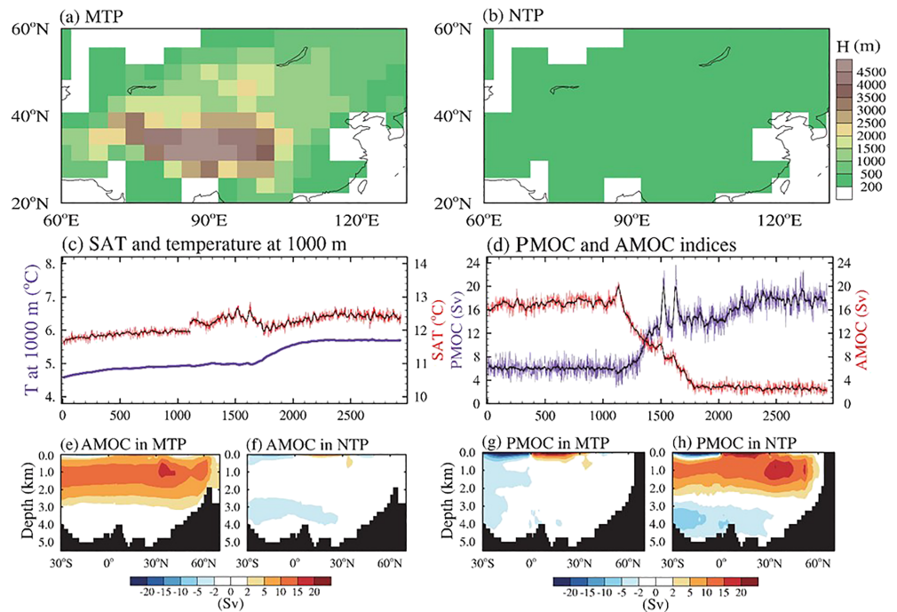
Figure 10. Two topographic height configurations used in experiments: (a) Modern Tibetan Plateau (MTP) and (b) No Tibetan Plateau (NTP), the elevation has been fixed to 200 m). (c) Time series of global mean annual 2-m surface air temperature (SAT) and sea temperature at 1,000 m depth in MTP (1–1,100 years) and NTP (1,101–2,940 years) simulations; bold black lines show the 21-year running mean. (d) Same as (c) but for PMOC and AMOC indices. AMOC and PMOC indices are defined as the annual maximum of the meridional stream function value north of 28°N and below the depth of 500 m over the North Atlantic and Pacific, respectively. (e–h) Climatological annual mean Atlantic and Indian-Pacific meridional overturning stream function in (e, g) MTP and (f, h) NTP; positive (negative) shading represents clockwise (counterclockwise) circulations.
