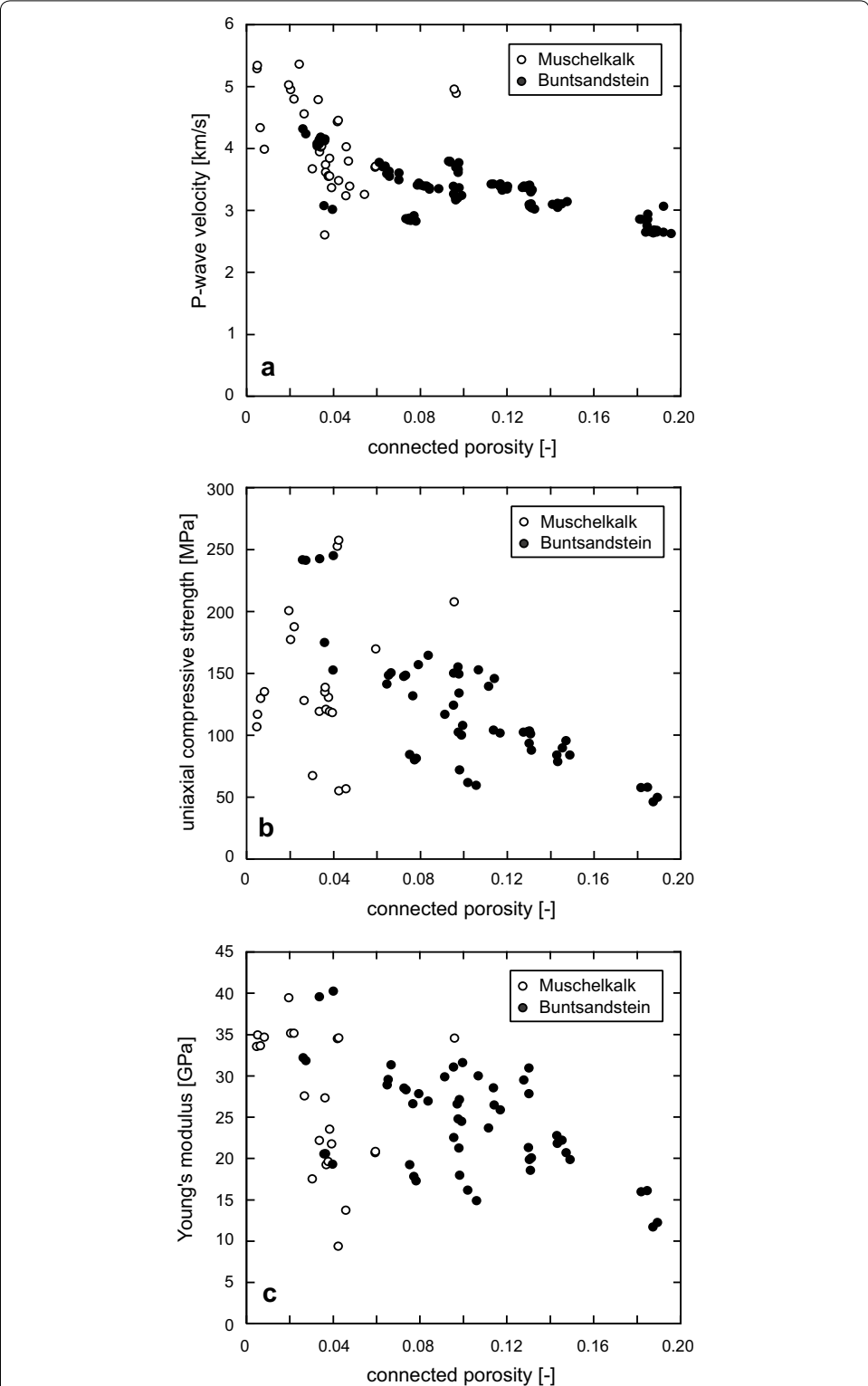
Fig. 10 a Dry P-wave velocity, b dry uniaxial compressive strength, and c dry Young's modulus as a function of connected porosity for Muschelkalk (white circles) and Buntsandstein (black circles) samples from exploration well EPS-1 (Soultz-sous-Forêts). Data for the Buntsandstein from this study and Heap et al. (2017, 2018, 2019)
