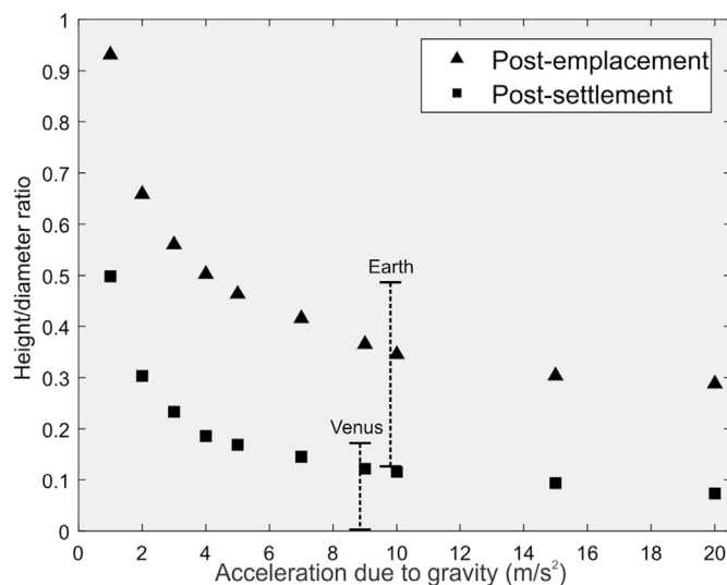
Fig. 2. Height/diameter ratio of a lava dome as a function of acceleration due to gravity for domes post-emplacment (triangles) and post-settlement (squares). Each symbol represents a unique model run. We note that macroscopic dome morphologies of model runs with the same input parameters are essentially identical and that any variability is captured by the symbol size. Height/diameter ratios for Earth and Venus are taken from Fink et al. (1993). Data for Earth is for Mt. St. Helens (USA) and Soufrière Hills volcano (Montserrat). Data for Venus includes “Class 1” and “Class 2” domes. We note that the height/diameter ratio ranges provided for Earth and Venus likely underestimate the true range.
