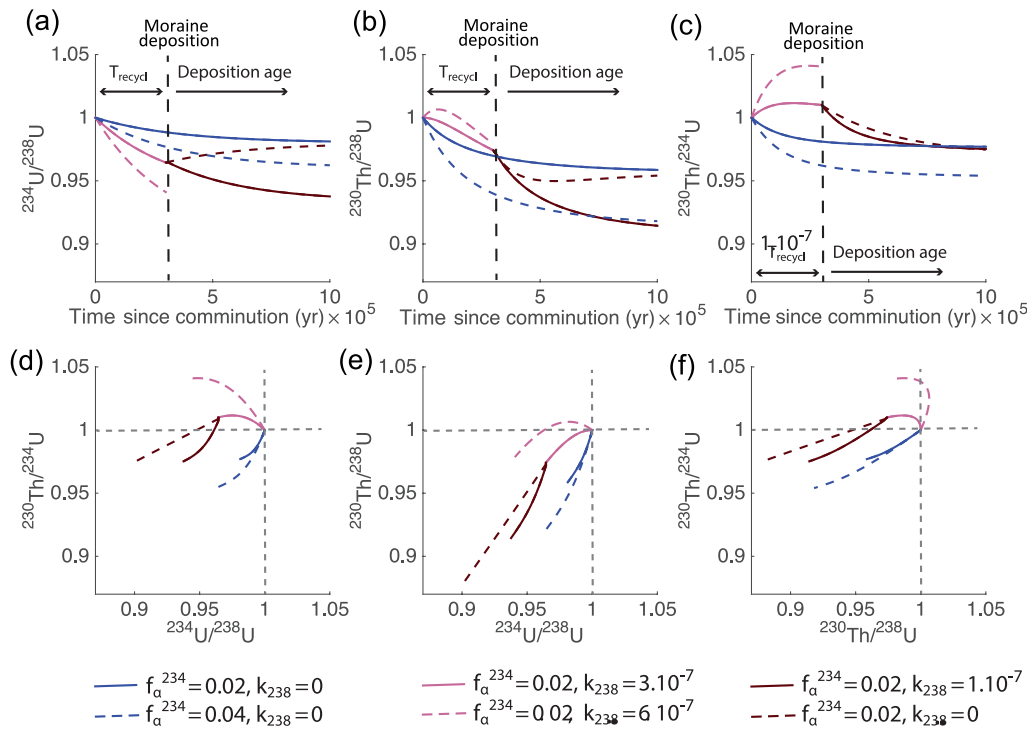
Figure 3. Solutions to Eq. 3 that we use as the theoretical framework to analyze our data for different values of f_{\alpha} and k_{238} (we consider k_{234}/k_{238} = 1.4 and k_{230}/k_{238} = 0.5 ). The time evolution of ^{234}\text{U}/^{238}\text{U} (a), ^{230}\text{Th}/^{238}\text{U} (b) and ^{230}\text{Th}/^{234}\text{U} (c) activity ratios. The vertical dashed line represents an event through which the weathering intensity varies: this corresponds in our case to the time of sediment remobilization. Our ^{10}\text{Be} exposure ages give the time elapsed since this event (shown by the dashed vertical line), whereas the U–Th data indicate the duration of the first phase since comminution and remobilization (from the x axis origin to the dashed vertical line). (d, e and f) The co-evolution of the ratios in (a), (b) and (c), respectively. Different scenarios are plotted corresponding to different f_{\alpha} values and weathering intensities to illustrate potential patterns in the comminution weathering model (see legend and Sect. 2.3.1). Observing these figures helps in understanding the range of variations in the different activity ratios and the effect of each parameter ( \alpha recoil and weathering) on these ratios before and after the remobilization of sediments.
