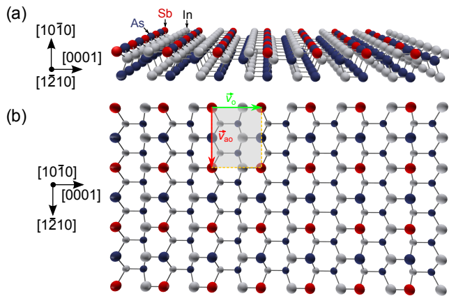
Figure 3. Perspective view of a ball model of the two-dimensional idealized (long range) chemical ordering of the monolayer shell on the InAs sidewall facet, based on the ordering and antiordering vectors extracted from pair correlation function. (a) Side and (b) top view with surface unit cell (gray shaded area) and ordering as well as anti ordering vectors shown as green and red arrows, respectively.
