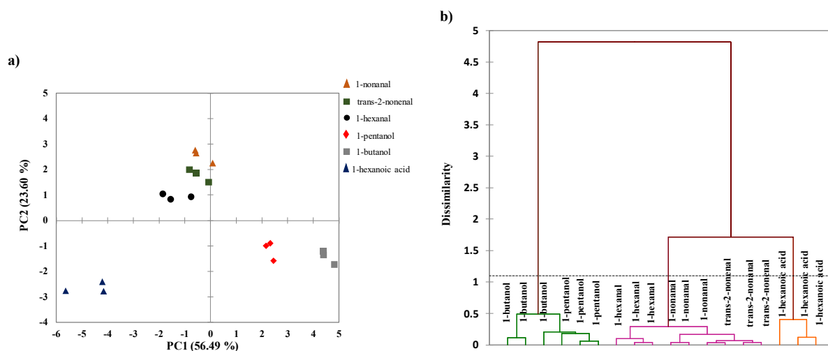
Fig. 6. a) PCA plots and b) AHC dendrograms for the discrimination of different VOCs by combining the responses of peptides with those of hpDNA.
