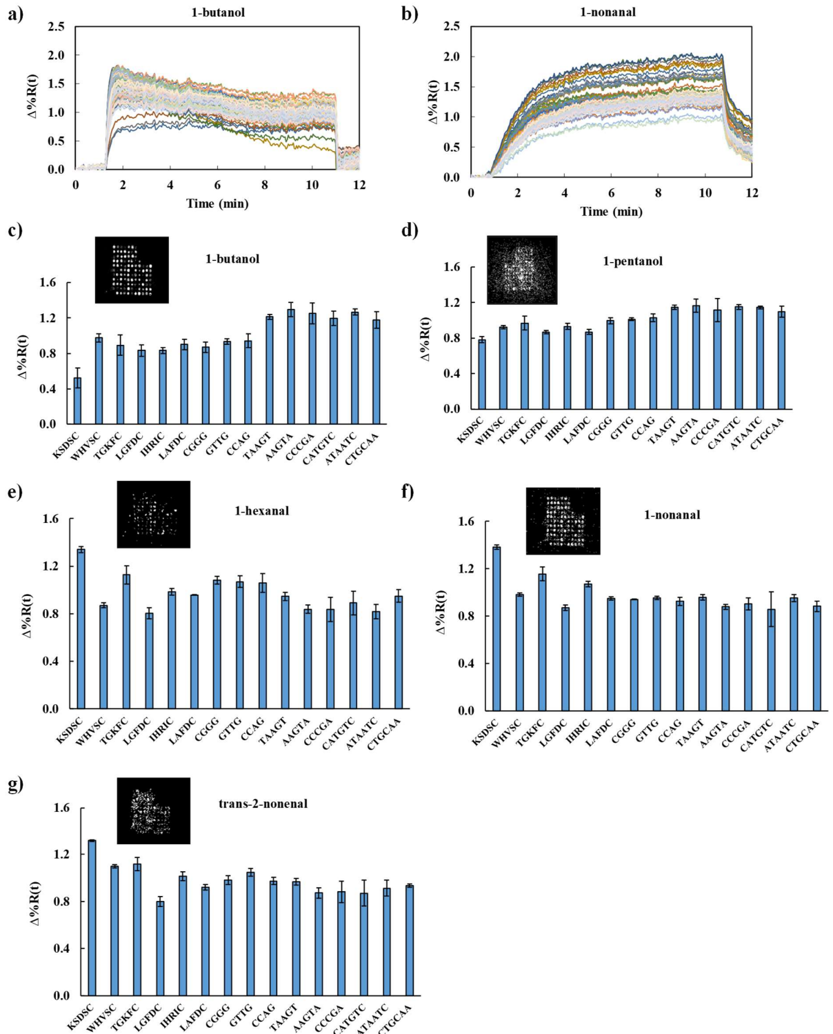
Fig. 2. Example of sensor responses after exposure to a) 1-butanol and b) 1-nonanal. Response patterns and characteristic SPRi images at equilibrium for c) 1-butanol (55 ppm), d) 1-pentanol (31 ppm), e) 1-hexanal (90 ppm), f) 1-nonanal (3.6 ppm) and g) trans-2-nonenal (7.0 ppm).
