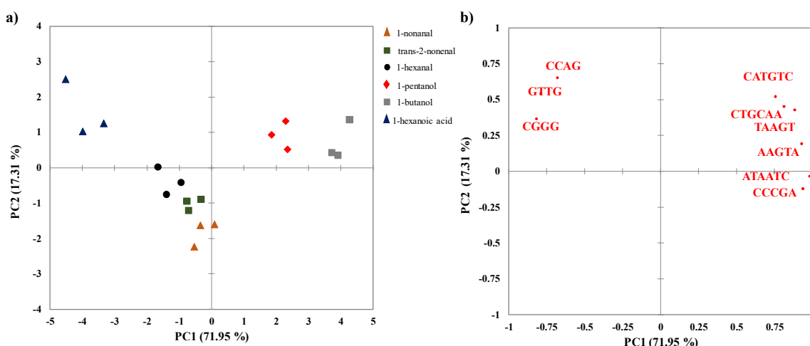
Fig. 4. PCA ( score and loading plots) for the discrimination of different VOCs with different hpDNA. In the left the score plot reporting VOCs analyzed. In the right the loadings plot reporting the contribution of the hpDNA with different loops (4; 5 and 6) reported in red.
