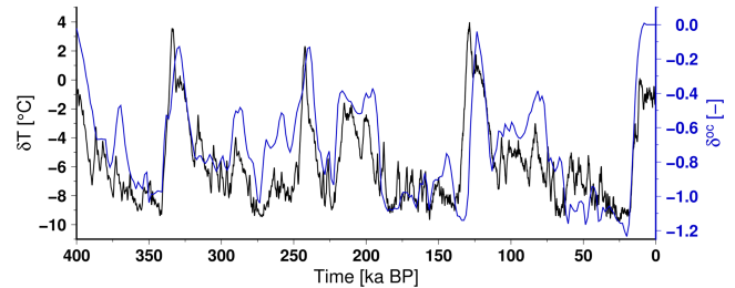
Figure 13. Climatic perturbation used in the 400 kyr glacial–interglacial simulations for the near-surface air temperature, \delta T = (1/\alpha^i) \delta D , and for the sub-shelf basal melting rate modifier, \delta^{\text{oc}} = \alpha^{\text{oc}} \Delta T_{\text{NA}}/T_{\text{NA0}} .
