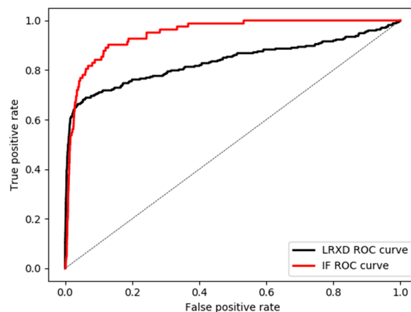
Figure 8. Receiver operating characteristic (ROC) curves for Isolation Forest (IF) and local Reed–Xiaoli detector (LRXD) anomaly detection calculated for the submerged structures.
