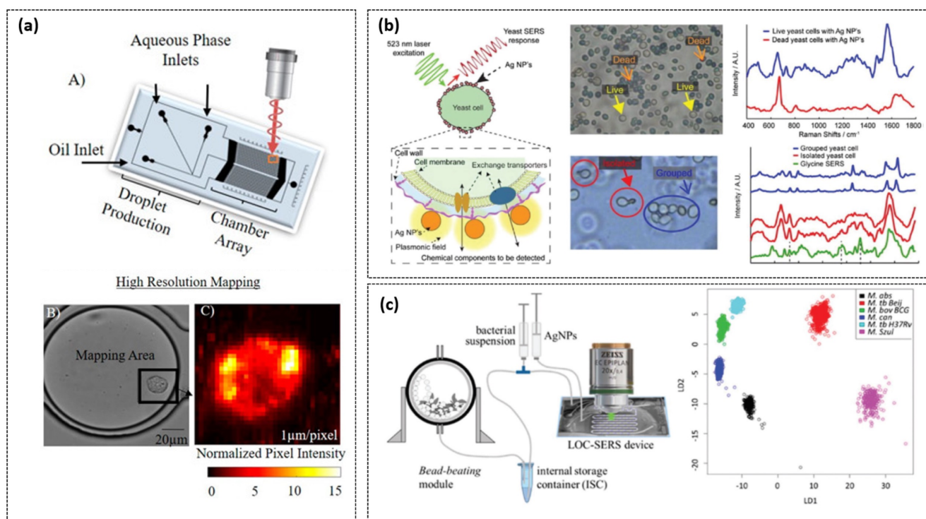
Fig. 3. Examples of MF-SERS applications in the biological field. (a) droplets-based single cell microfluidics strategy coupled to SERS to investigated glycan expression in cancer cells at cellular resolution (adapted from [76] with permission from American Chemical Society), (b) scheme of a MF-SERS set-up and comparison results of both live and dead cell and isolated and grouped yeasts cells (adapted from [78] with permission from Elsevier B.V.). (c) MF-SERS set-up and results for the identification of six different mycobacteria from blood samples (adapted with permission from [79] with permission from American Chemical Society).
