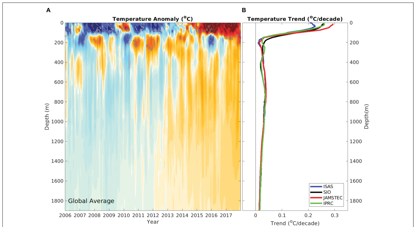
FIGURE 12 | (A) Global averaged temperature anomaly ( ^{\circ}\text{C} – from SIO) and (B) trend ( ^{\circ}\text{C}/\text{decade} , 2006–2018) versus depth, based on gridded Argo data. Gridded product sources are: ISAS (Gaillard et al., 2016), SIO (Roemmich and Gilson, 2009); IPRC- from the Asia-Pacific Data Research Center ( http://apdrc.soest.hawaii.edu/projects/Argo/data/gridded/On_standard_levels/index-1.html ); JAMSTEC (Hosoda et al., 2008).
