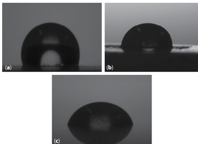
Figure 3 Wettability variations of CPEs studied determined by contact angle measurements A = CPE; B = CPE-CHr, C = CPE-Ce ( pH of the water deposited 6.5, technic: sessile drop; droplet volume 2 mL; temperature: 22 °C ).
