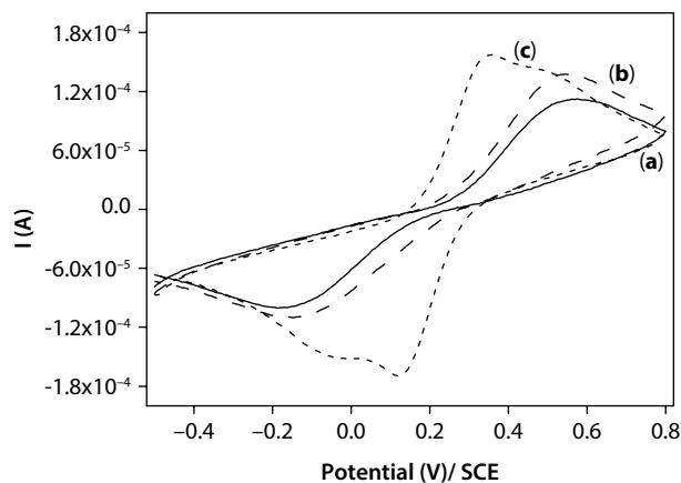
Figure 4 Cyclic voltammograms of 5 mM [\text{Fe}(\text{CN})_6]^{3-} solution in 0.1 M \text{KNO}_3 at the (a) bare CPE, (b) CPE-CHr and (c) CPE-Ce. Potential scan rate: 100 mV s -1 .
