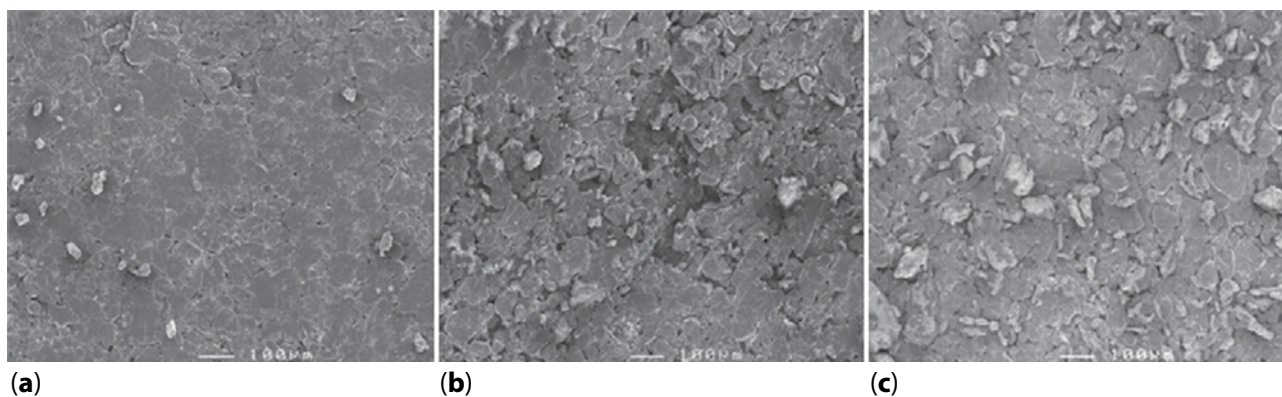
Figure 1 2D-SEM images of bare CPE (a), CPE-CHr (b) and CPE-Ce (c).
