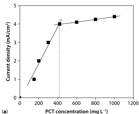
(a) Evolution of peak current densities vs. PCT concentration at CPE-CHr.
