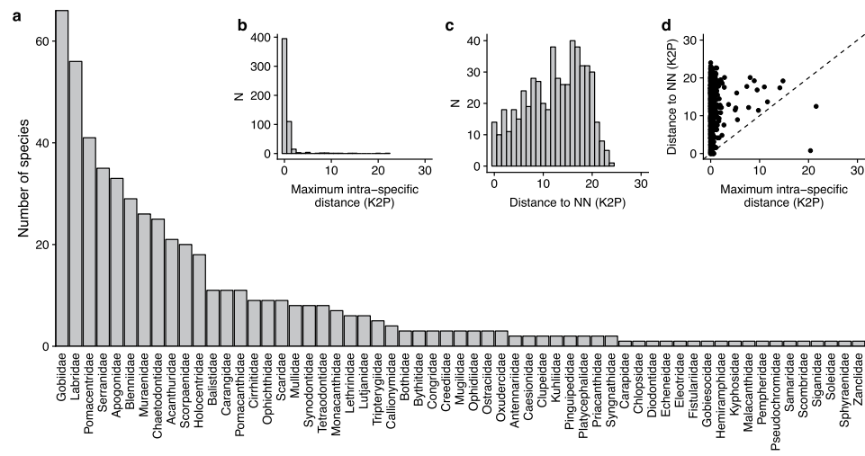
Fig. 3 Species diversity and distribution of genetic distance across the DNA barcode library. (a) Species diversity by family for the four archipelagos sampled; (b) Distribution of maximum intraspecific distances (K2P, percent); (c) Distribution of nearest neighbor distances (K2P, percent); (d) Relationship between maximum intraspecific and nearest neighbor distances. Points above the diagonal line indicate species with a barcode gap.
