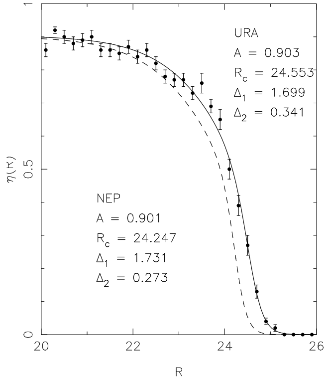
Figure 3. The TNO detection efficiency as a function of R-band magnitude for the two halves of the survey. Dashed curve: best fit to the TNO efficiency near Neptune. Solid curve and points: Efficiency data and best fit for the fields taken near Uranus. The quality of the fit to the efficiency data points near Neptune (not shown) is comparable to that near Uranus. The best fit parameters to the functional form of Eq. 2 is given. The fields near Uranus are roughly 0.3 magnitudes deeper due to the consistently better seeing in the second halves of our nights.
